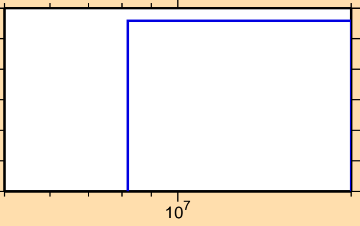
\sigma vs. E for ^{108}\text{Rh}(n,\text{nd})
