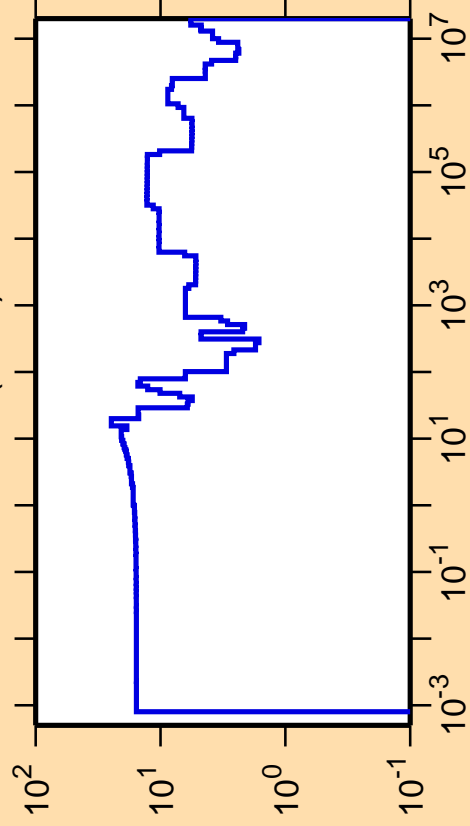
\Delta\sigma/\sigma vs. E for ^{109}\text{Rh}(n,\text{el.})
