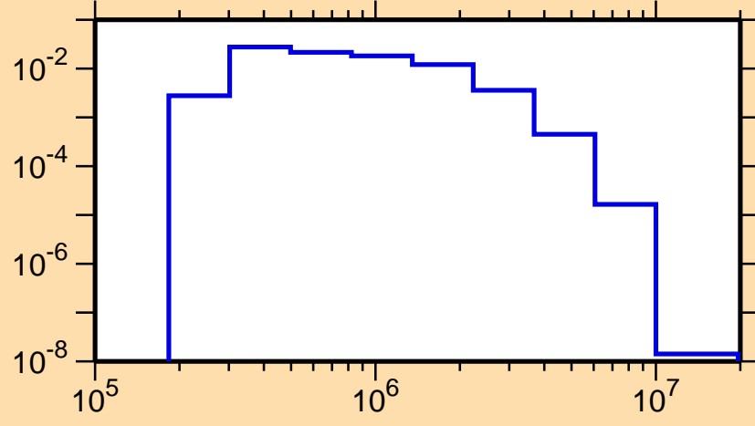
\sigma vs. E for ^{109}\text{Rh}(n,n_3)
