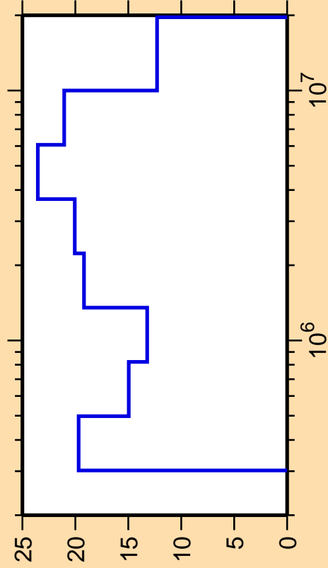
\Delta\sigma/\sigma vs. E for ^{109}\text{Rh}(n,n_4)
