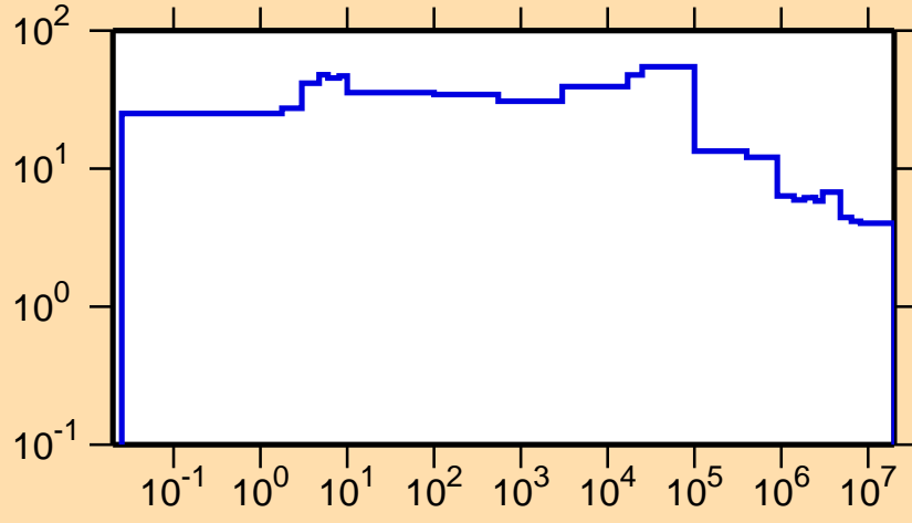
\Delta\sigma/\sigma vs. E for ^{109}\text{Rh}(n,\text{nonel.})
