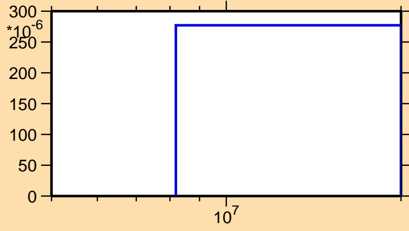
\sigma vs. E for ^{109}\text{Rh}(n,np)
