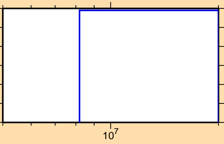
\sigma vs. E for ^{109}\text{Rh}(n,2np)
