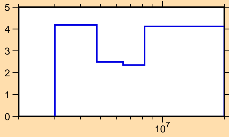
\Delta\sigma/\sigma vs. E for ^{109}\text{Rh}(n,\text{el.})
