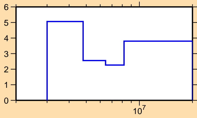
\Delta\sigma/\sigma vs. E for ^{109}\text{Rh}(n,\text{tot.})
