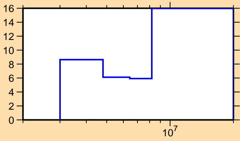
\Delta\sigma/\sigma vs. E for ^{109}\text{Rh}(n,n\text{cont.})
