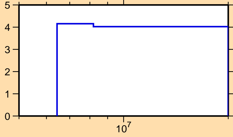
\Delta\sigma/\sigma vs. E for ^{109}\text{Rh}(n,\text{nonel.})
