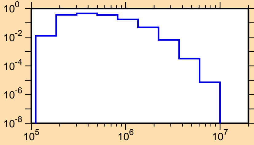
\sigma vs. E for ^{110}\text{Rh}(n,n_2)
