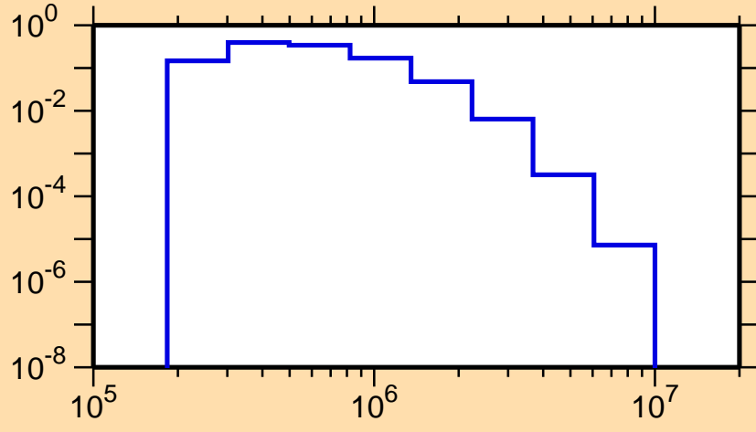
\sigma vs. E for ^{110}\text{Rh}(n,n_3)
