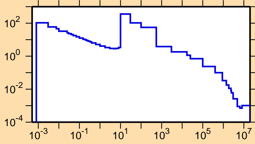
\sigma vs. E for ^{110}\text{Rh}(n,\gamma)
