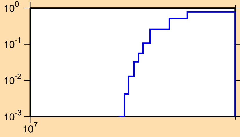
\sigma vs. E for ^{111}\text{Rh}(n,3n)
