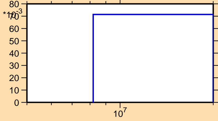
\sigma vs. E for ^{111}\text{Rh}(n,3n)
