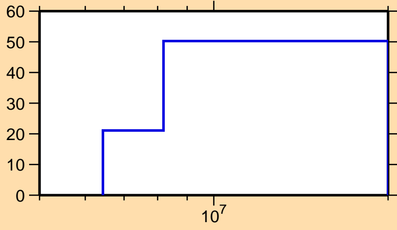
\Delta\sigma/\sigma vs. E for ^{111}\text{Rh}(n,n\text{cont.})
