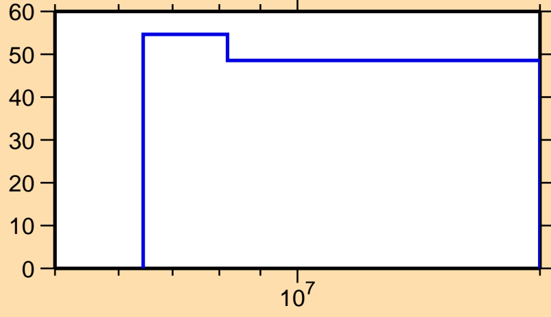
\Delta\sigma/\sigma vs. E for ^{111}\text{Rh}(n,n_1)
