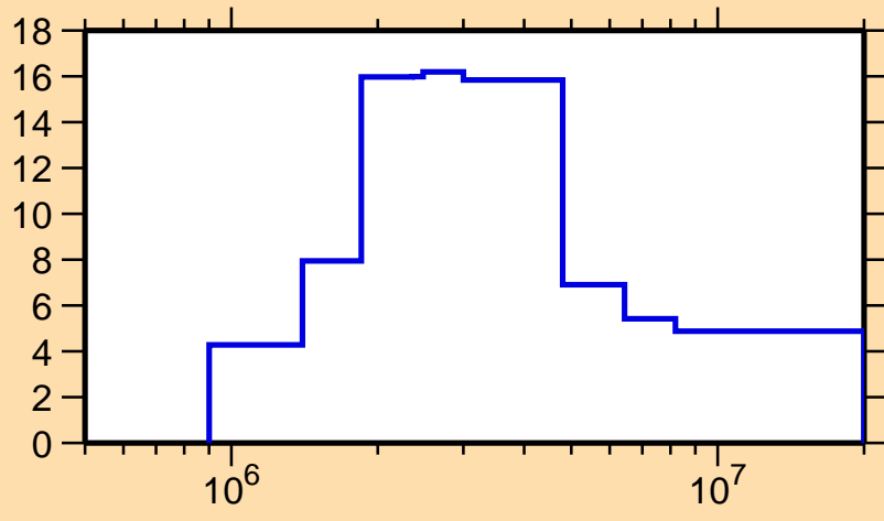
\Delta\sigma/\sigma vs. E for ^{111}\text{Rh}(n,\text{tot.})
