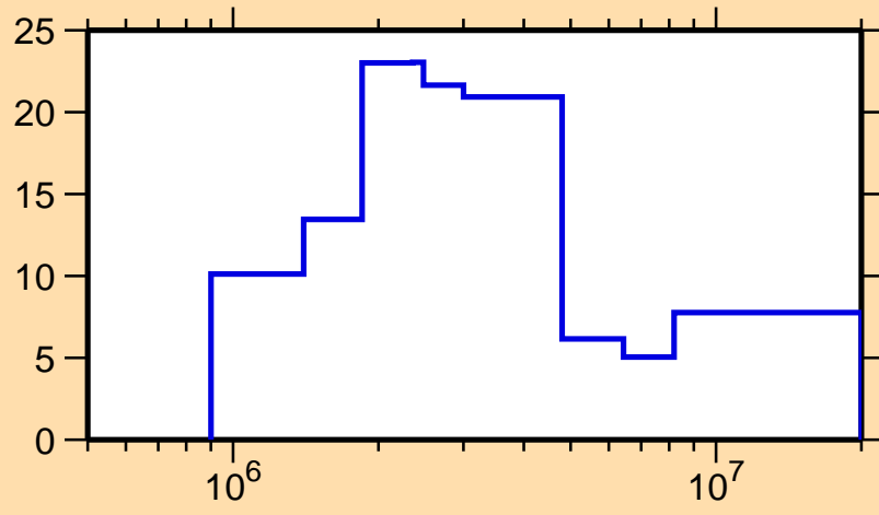
\Delta\sigma/\sigma vs. E for ^{111}\text{Rh}(n,\text{el.})
