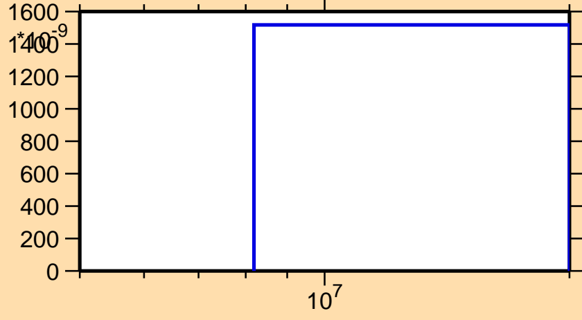
\sigma vs. E for ^{111}\text{Rh}(n,n\alpha)
