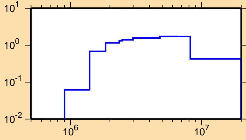
\sigma vs. E for ^{111}\text{Rh}(n,n\text{cont.})
