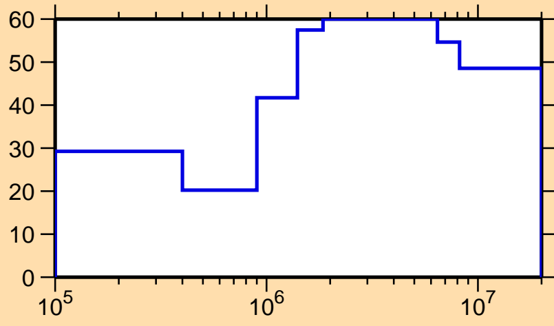
\Delta\sigma/\sigma vs. E for ^{111}\text{Rh}(n,n_1)
