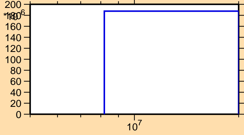
\sigma vs. E for ^{111}\text{Rh}(n,d)
