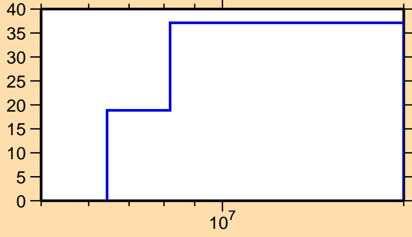
\Delta\sigma/\sigma vs. E for ^{111}\text{Rh}(n,\text{inel.})
