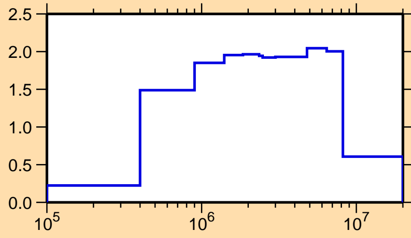
\sigma vs. E for ^{111}\text{Rh}(n,\text{inel.})
