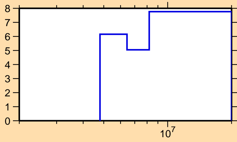
\Delta\sigma/\sigma vs. E for ^{111}\text{Rh}(n,\text{el.})
