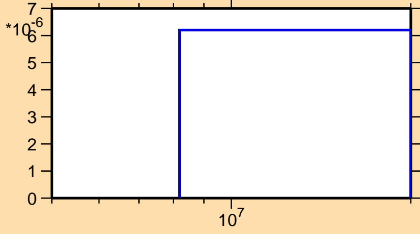
\sigma vs. E for ^{111}\text{Rh}(n,t)
