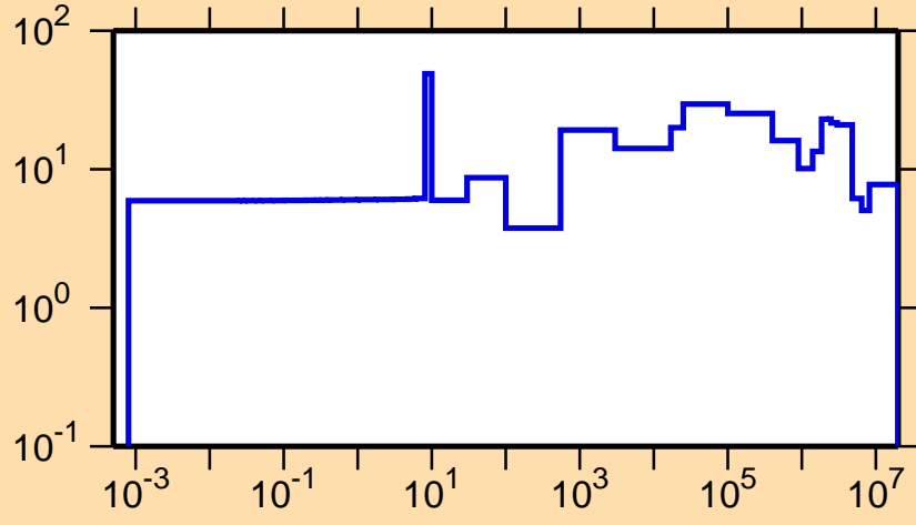
\Delta\sigma/\sigma vs. E for ^{111}\text{Rh}(n,\text{el.})
