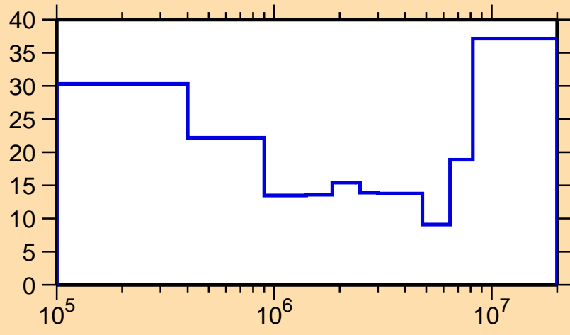
\Delta\sigma/\sigma vs. E for ^{111}\text{Rh}(n,\text{inel.})
