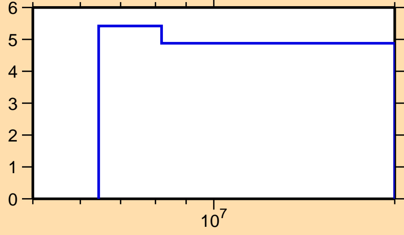
\Delta\sigma/\sigma vs. E for ^{111}\text{Rh}(n,\text{tot.})
