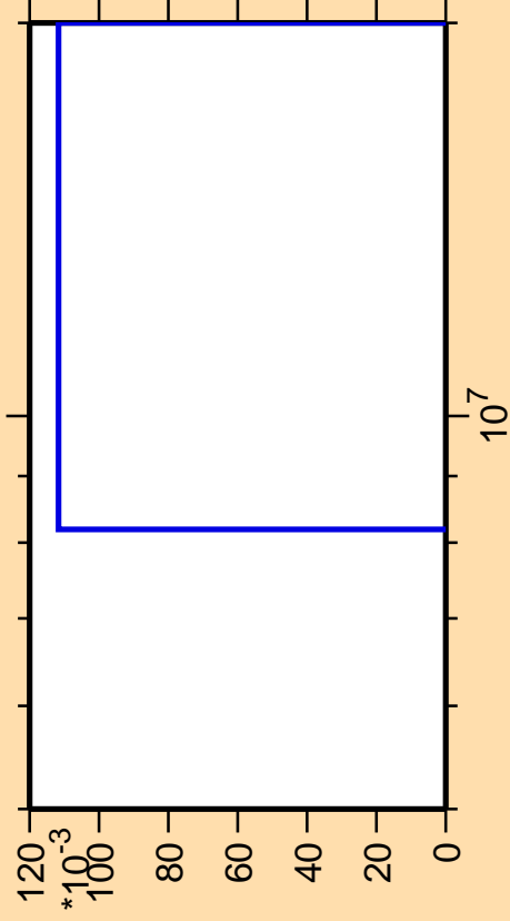
\Delta\sigma/\sigma vs. E for ^{111}\text{Rh}(n,2n\alpha)
