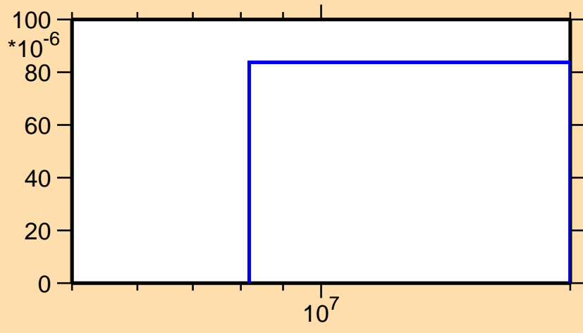
\sigma vs. E for ^{111}\text{Rh}(n,np)
