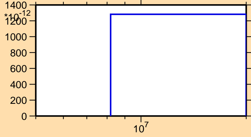
\sigma vs. E for ^{111}\text{Rh}(n,\text{nd})
