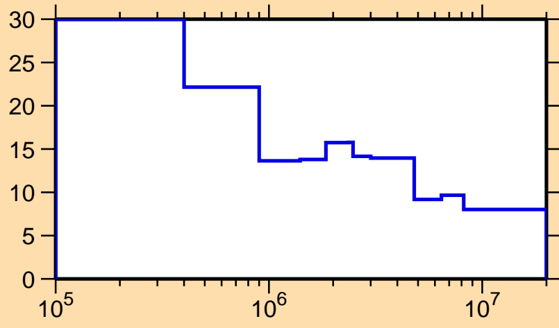
\Delta\sigma/\sigma vs. E for ^{111}\text{Rh}(n,\text{nonel.})
