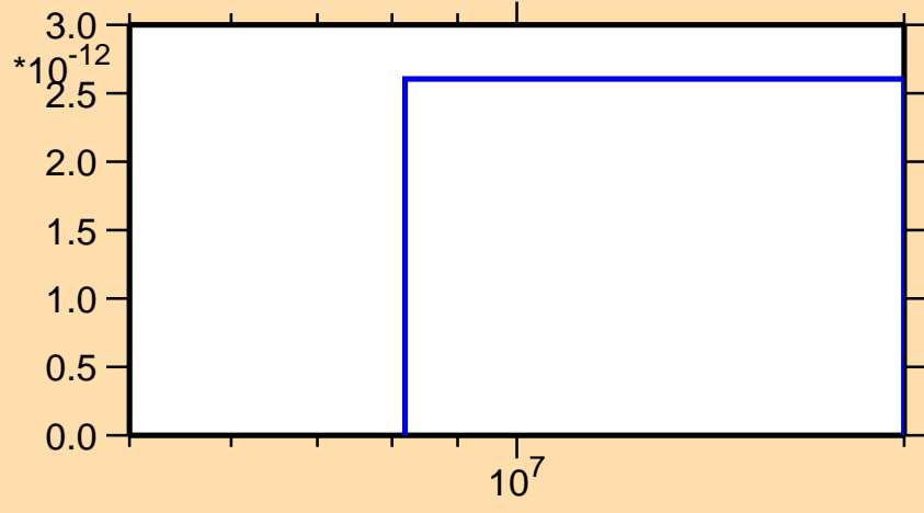
\sigma vs. E for ^{111}\text{Rh}(n,2np)
