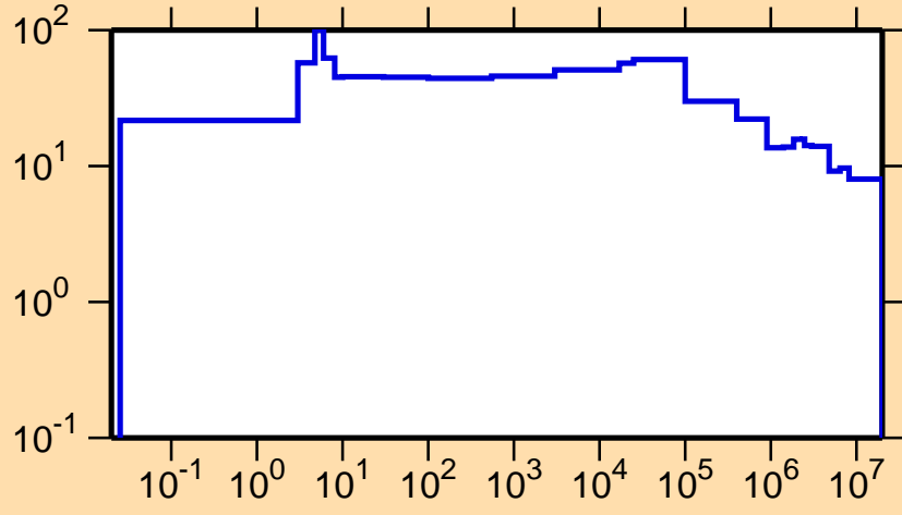
\Delta\sigma/\sigma vs. E for ^{111}\text{Rh}(n,\text{nonel.})
