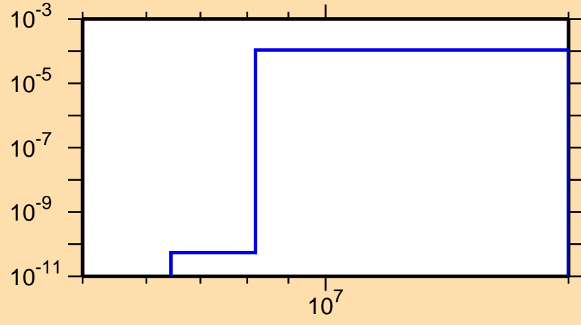
\sigma vs. E for ^{111}\text{Rh}(n,\alpha)
