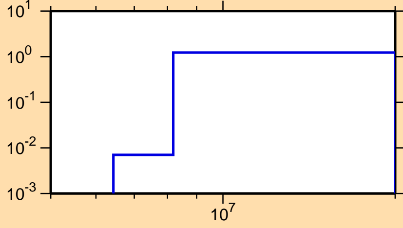
\sigma vs. E for ^{111}\text{Rh}(n,2n)
