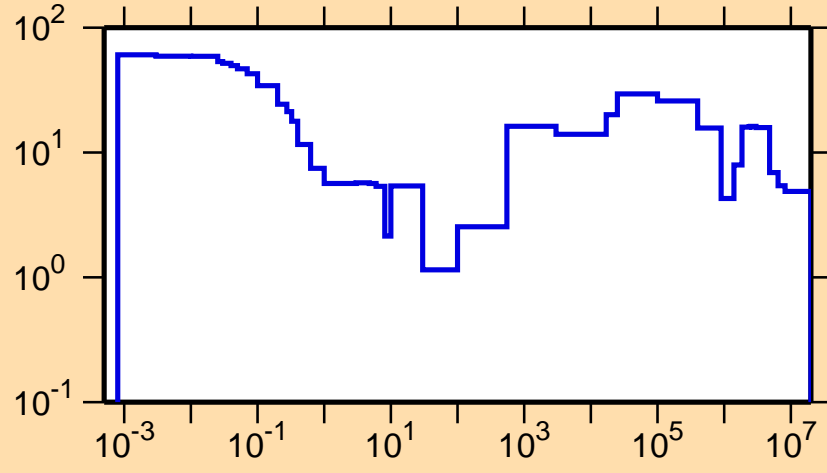
\Delta\sigma/\sigma vs. E for ^{111}\text{Rh}(n,\text{tot.})
