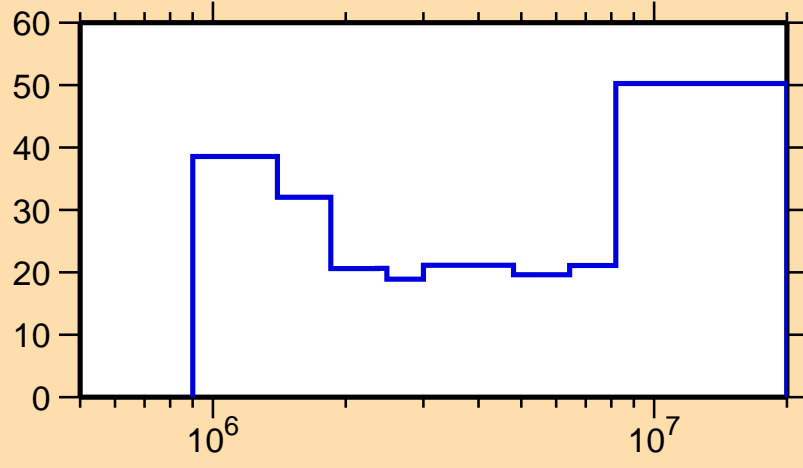
\Delta\sigma/\sigma vs. E for ^{111}\text{Rh}(n,n\text{cont.})
