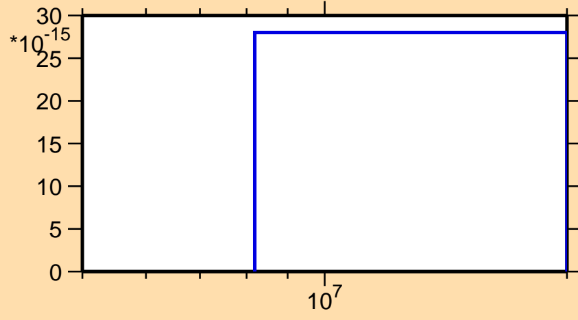
\sigma vs. E for ^{111}\text{Rh}(n,2n\alpha)
