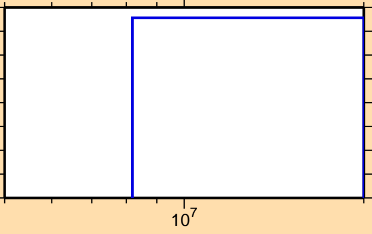
\sigma vs. E for ^{111}\text{Rh}(n,nt)
