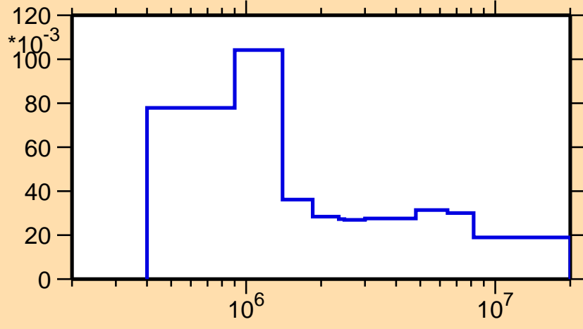
\sigma vs. E for ^{112}\text{Rh}(n,n_1)
