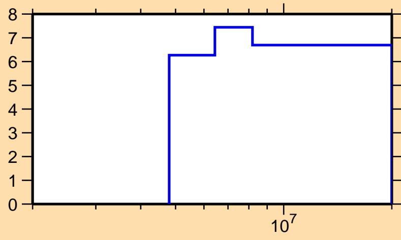
\Delta\sigma/\sigma vs. E for ^{112}\text{Rh}(n,\text{nonel.})
