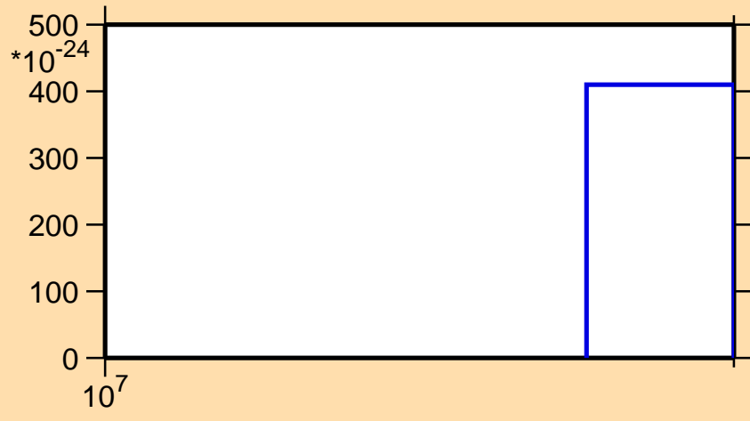
\sigma vs. E for ^{112}\text{Rh}(\text{mt } 11)
