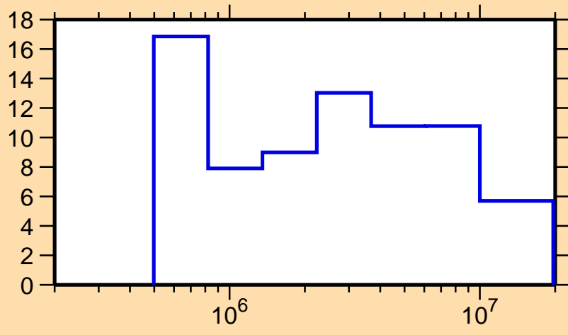
\Delta\sigma/\sigma vs. E for ^{112}\text{Rh}(n, el.)
