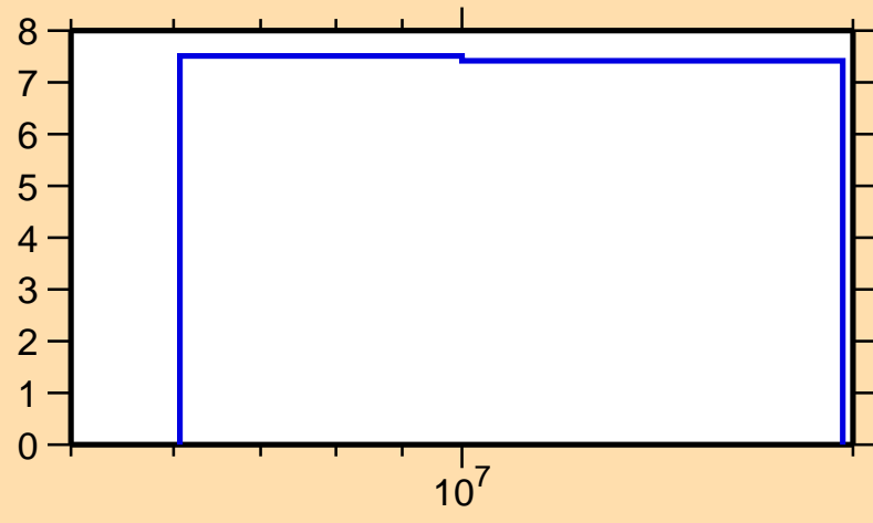
\Delta\sigma/\sigma vs. E for ^{113}\text{Rh}(n,\text{el.})
