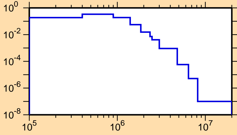
\sigma vs. E for ^{114}\text{Rh}(n,n_2)
