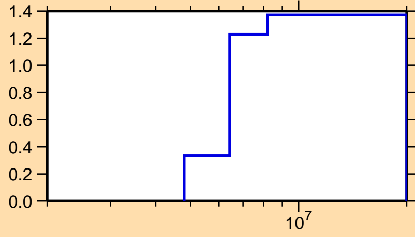
\sigma vs. E for ^{114}\text{Rh}(n,2n)
