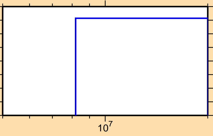
\sigma vs. E for ^{114}\text{Rh}(n,t)
