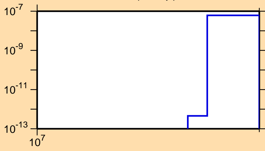
\sigma vs. E for ^{114}\text{Rh}(n,2np)
