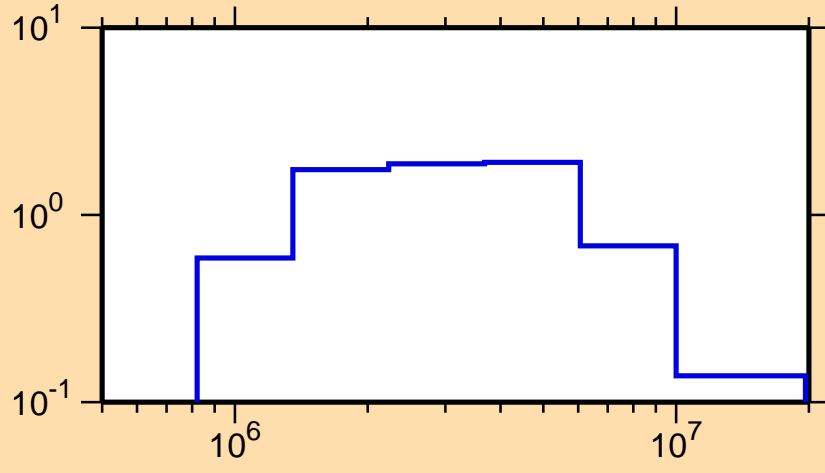
\sigma vs. E for ^{114}\text{Rh}(n,n\text{cont.})
