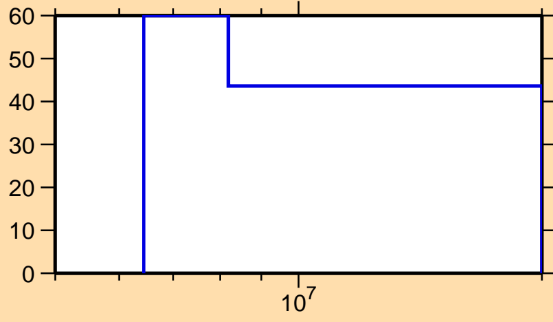
\Delta\sigma/\sigma vs. E for ^{114}\text{Rh}(n,ncont.)
