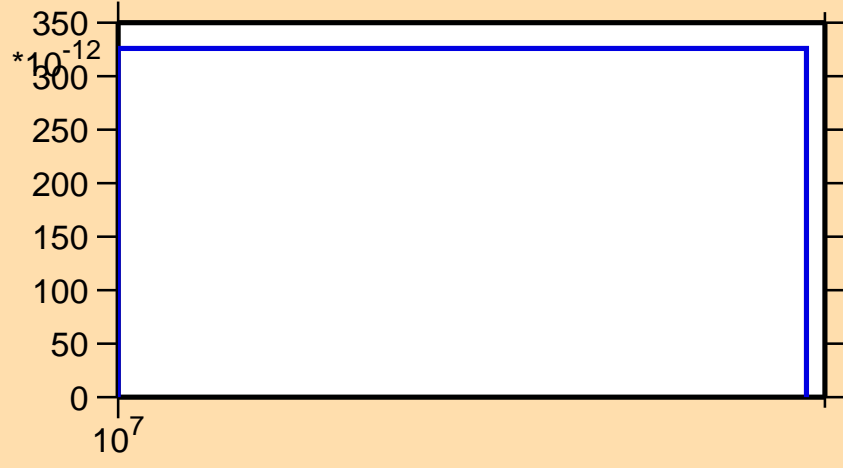
\sigma vs. E for ^{200}\text{Rn}(n,2np)
