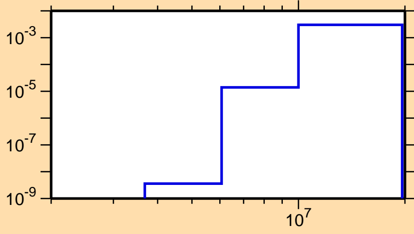
\sigma vs. E for ^{200}\text{Rn}(n,np)
