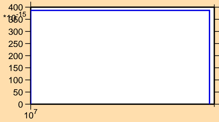
\sigma vs. E for ^{200}\text{Rn} (mt 34)
