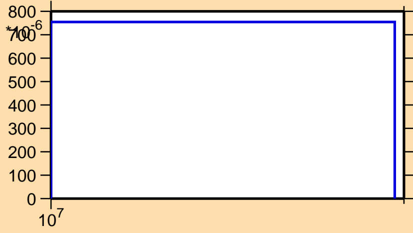
\sigma vs. E for ^{200}\text{Rn}(n,2n)
