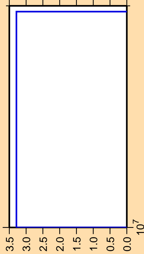
\Delta\sigma/\sigma vs. E for ^{200}\text{Rn} (mt 34)
