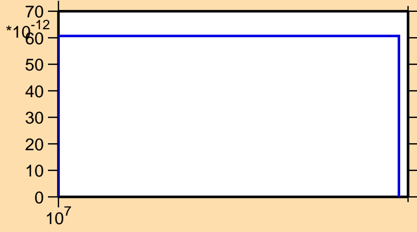
\sigma vs. E for ^{200}\text{Rn}(n,pt)
