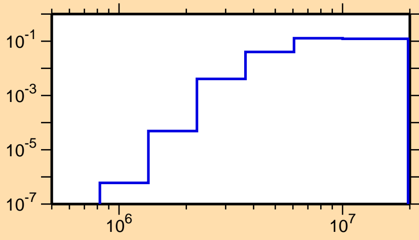
\sigma vs. E for ^{200}\text{Rn}(n,n\text{cont.})
