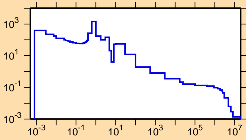
\sigma vs. E for ^{200}\text{Rn}(n,\gamma)
