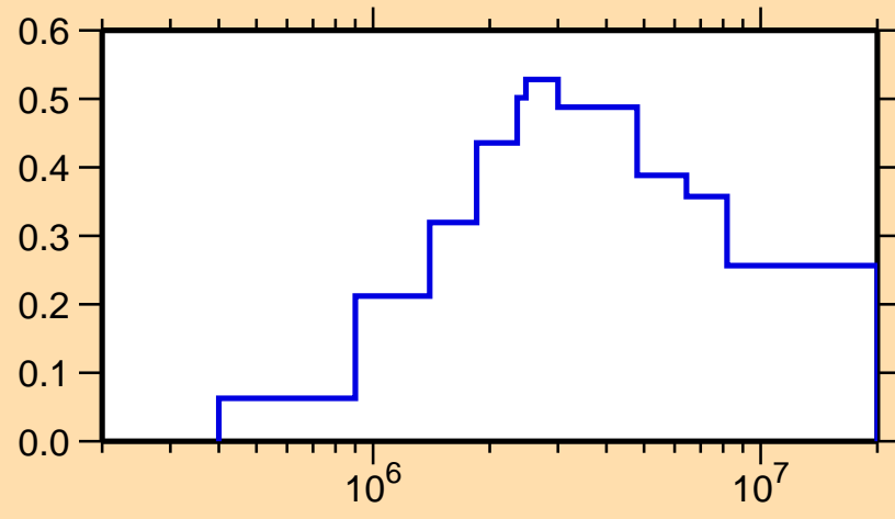
\sigma vs. E for ^{200}\text{Rn}(n,\text{inel.})
