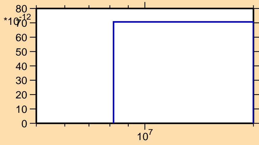
\sigma vs. E for ^{200}\text{Rn}(n,nd)
