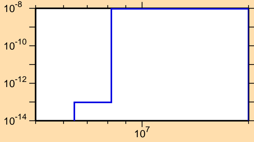
\sigma vs. E for ^{200}\text{Rn}(\text{mt117})
