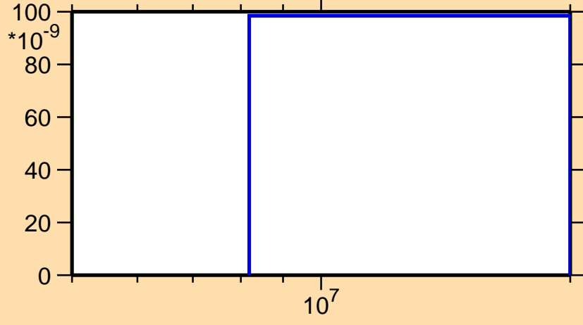
\sigma vs. E for ^{200}\text{Rn}(n,\text{pd})
