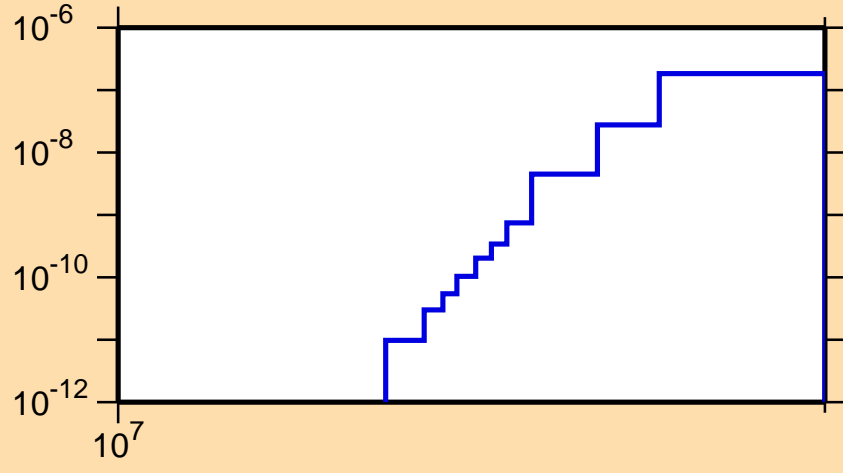
\sigma vs. E for ^{201}\text{Rn}(n,\text{pt})
