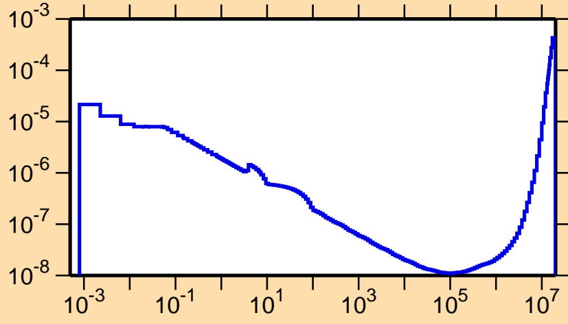
\sigma vs. E for ^{201}\text{Rn}(n,p\alpha)
