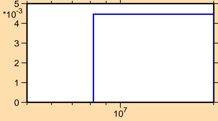
\sigma vs. E for ^{201}\text{Rn}(n,2n)
