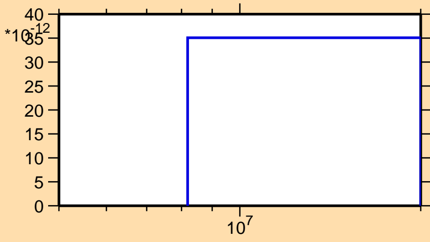
\sigma vs. E for ^{201}\text{Rn}(\text{mt } 34)
