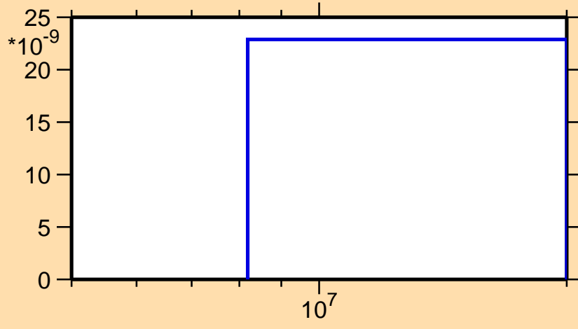
\sigma vs. E for ^{201}\text{Rn}(\text{mt } 45)
