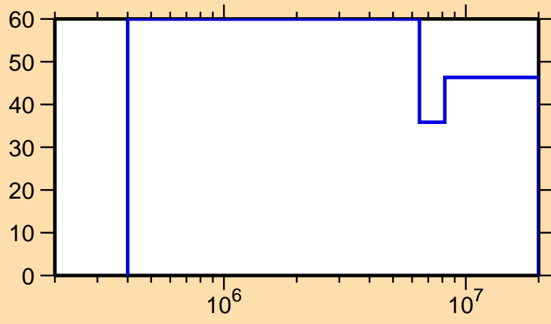
\Delta\sigma/\sigma vs. E for ^{201}\text{Rn}(n,n\text{cont.})
