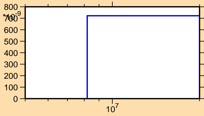
\sigma vs. E for ^{201}\text{Rn}(n,2n\alpha)
