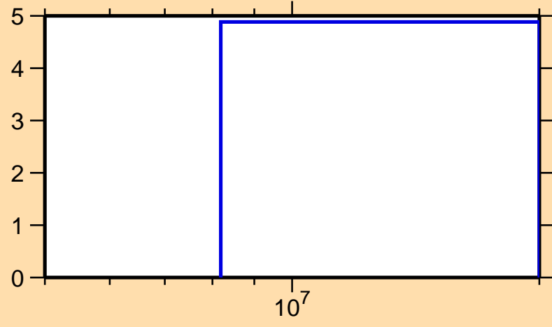
\Delta\sigma/\sigma vs. E for ^{201}\text{Rn}(n,\text{el.})
