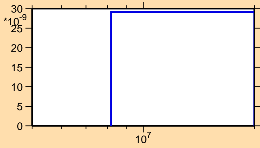
\sigma vs. E for ^{201}\text{Rn}(n,\text{pd})
