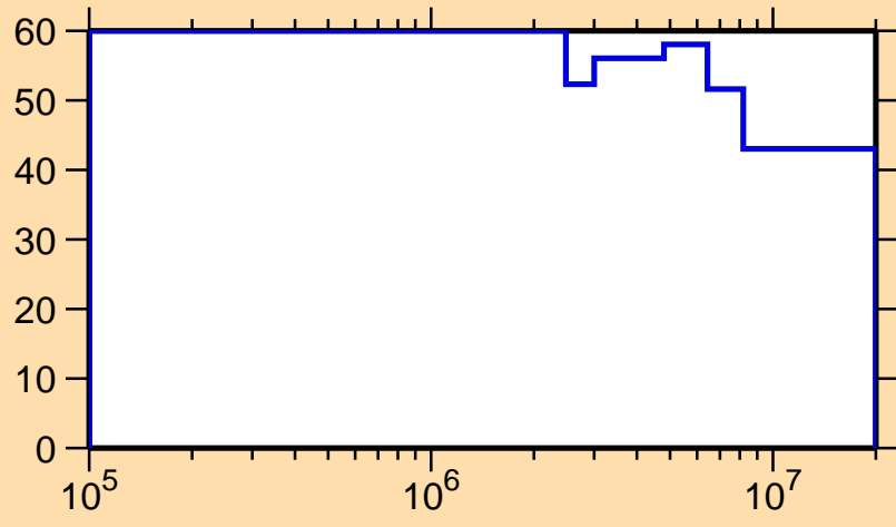
\Delta\sigma/\sigma vs. E for ^{201}\text{Rn}(n,n_1)
