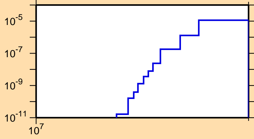
\sigma vs. E for ^{201}\text{Rn}(n,2np)
