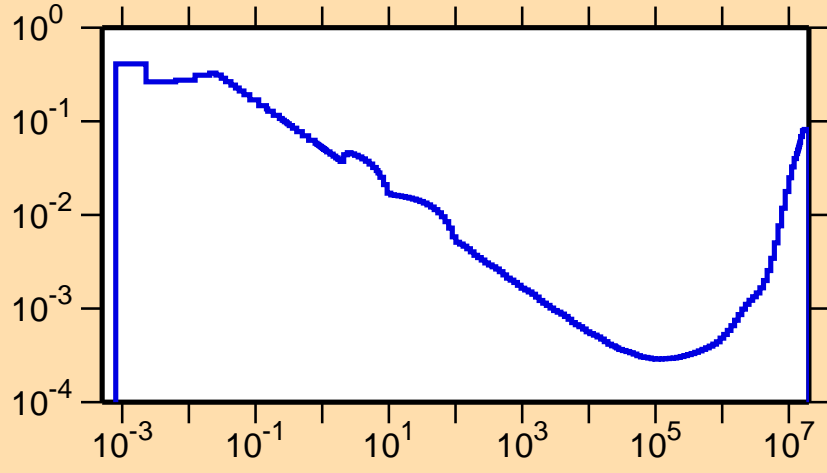
\sigma vs. E for ^{201}\text{Rn}(n,\alpha)
