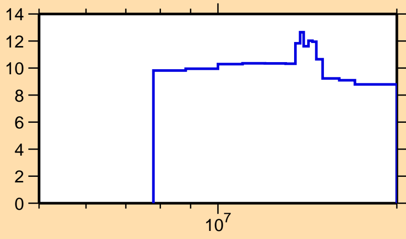
\Delta\sigma/\sigma vs. E for ^{201}\text{Rn}(n,\text{nonel.})
