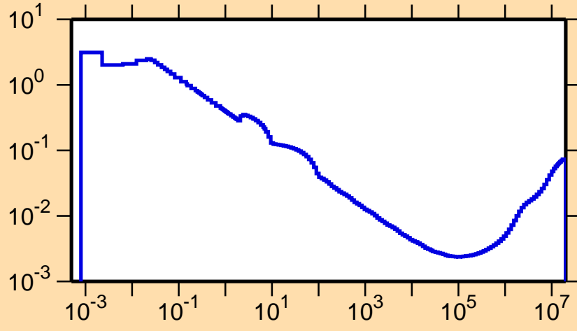
\sigma vs. E for ^{201}\text{Rn}(n,p)
