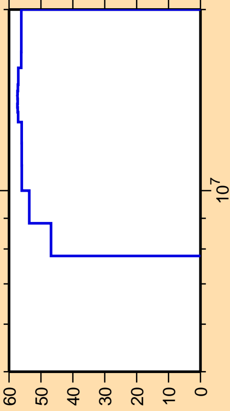
\Delta\sigma/\sigma vs. E for ^{201}\text{Rn}(n,n\text{cont.})
