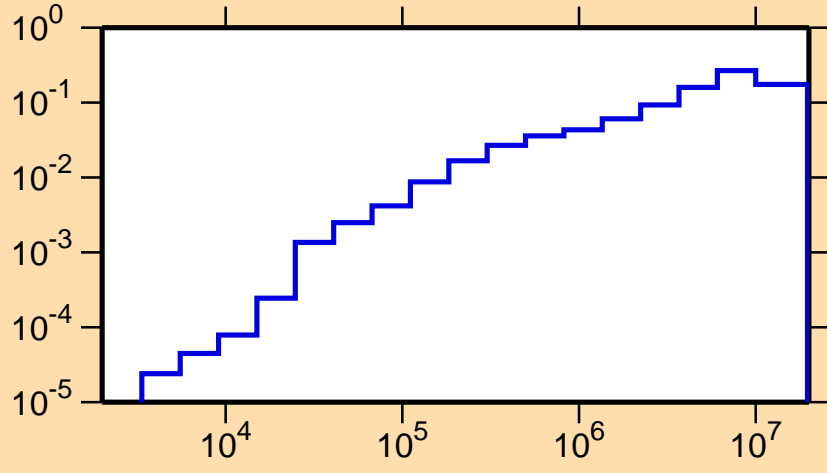
\sigma vs. E for ^{201}\text{Rn}(n,n\text{cont.})
