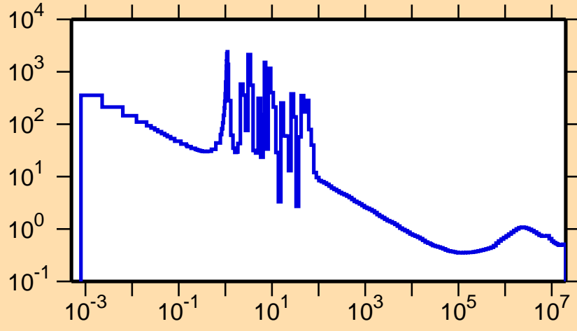
\sigma vs. E for ^{202}\text{Rn}(n,\text{nonel.})
