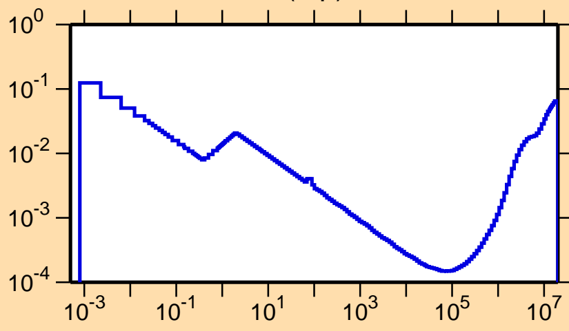
\sigma vs. E for ^{202}\text{Rn}(n,p)
