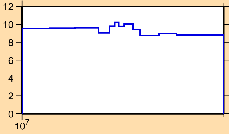
\Delta\sigma/\sigma vs. E for ^{202}\text{Rn}(n,\text{nonel.})
