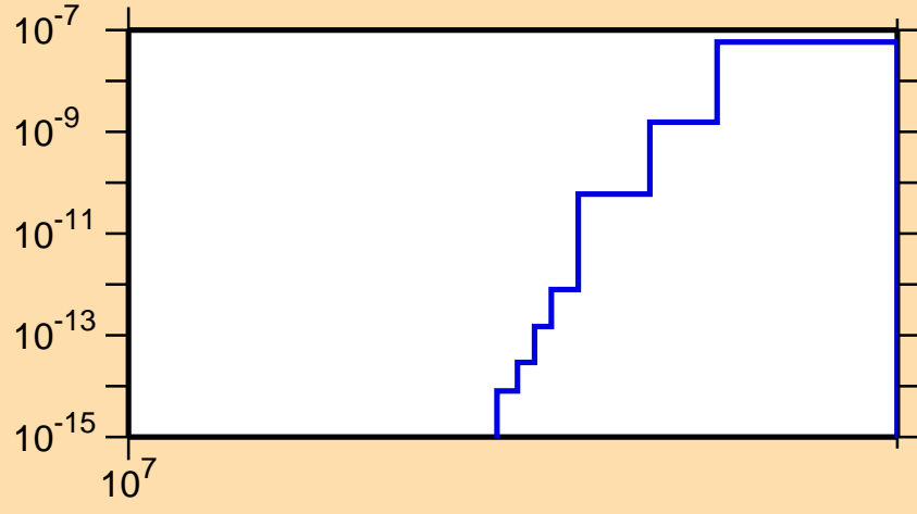
\sigma vs. E for ^{202}\text{Rn}(n,nd)
