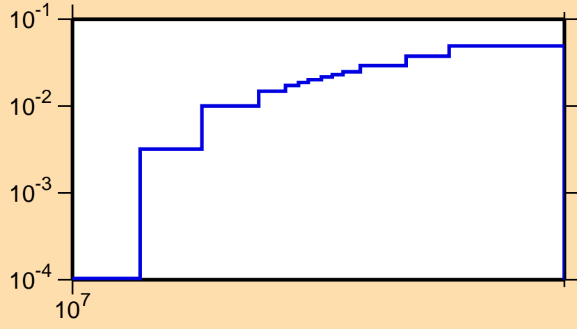
\sigma vs. E for ^{202}\text{Rn}(n,2n)
