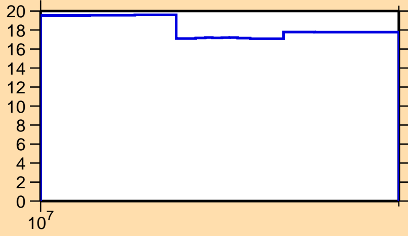
\Delta\sigma/\sigma vs. E for ^{202}\text{Rn}(n,\text{inel.})
