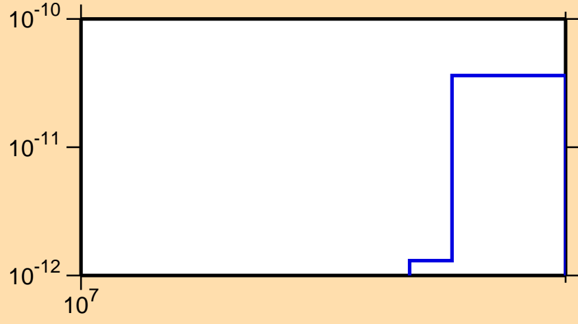
\sigma vs. E for ^{202}\text{Rn} (mt 34)
