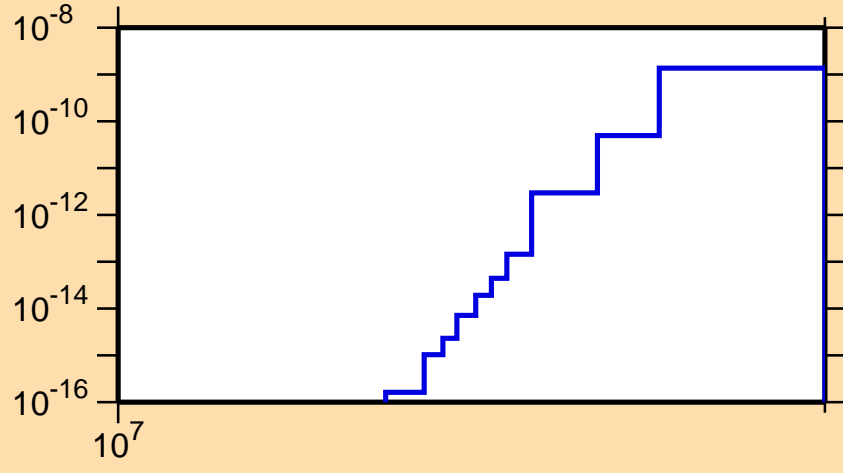
\sigma vs. E for ^{202}\text{Rn}(n,pt)
