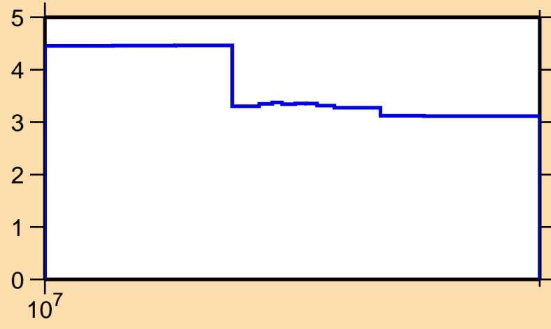
\Delta\sigma/\sigma vs. E for ^{202}\text{Rn}(n,\text{tot.})
