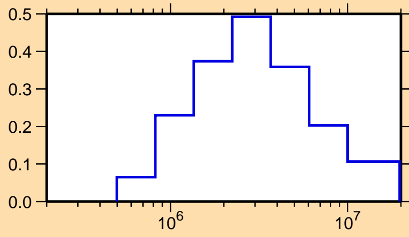
\sigma vs. E for ^{202}\text{Rn}(n,n_1)
