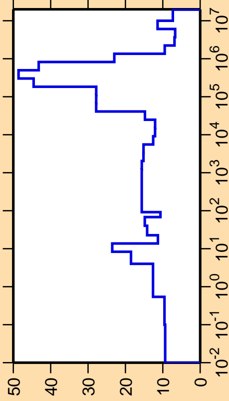
\Delta\sigma/\sigma vs. E for ^{202}\text{Rn}(n,\text{el.})
