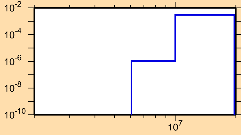
\sigma vs. E for ^{202}\text{Rn}(n,d)
