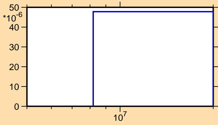
\sigma vs. E for ^{202}\text{Rn}(n,t)
