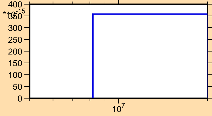
\sigma vs. E for ^{202}\text{Rn}(\text{mt } 34)
