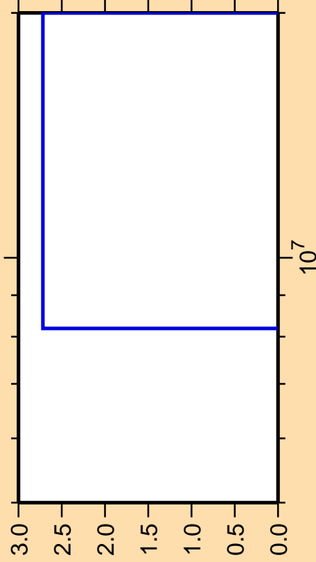
\Delta\sigma/\sigma vs. E for ^{202}\text{Rn}(\text{mt } 34)
