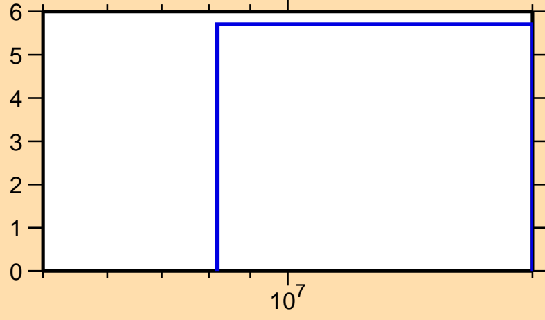
\Delta\sigma/\sigma vs. E for ^{202}\text{Rn}(n,\text{el.})
