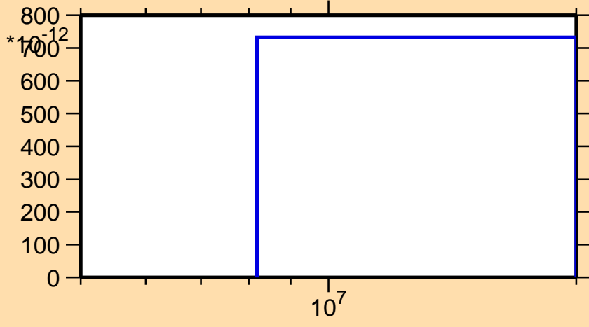
\sigma vs. E for ^{202}\text{Rn}(n,3n)
