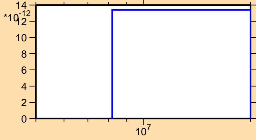
\sigma vs. E for ^{202}\text{Rn}(n,\text{pt})
