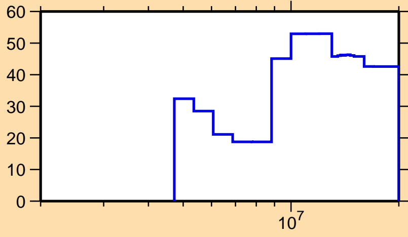
\Delta\sigma/\sigma vs. E for ^{203}\text{Rn}(n,n\text{cont.})
