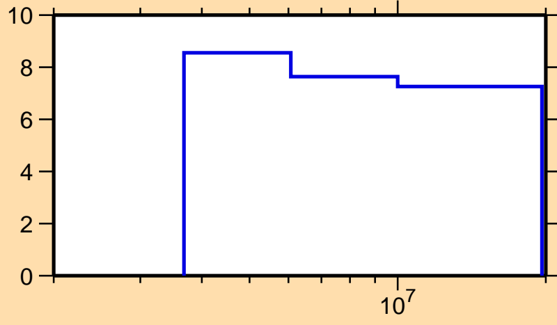
\Delta\sigma/\sigma vs. E for ^{203}\text{Rn}(n,n\text{onel.})
