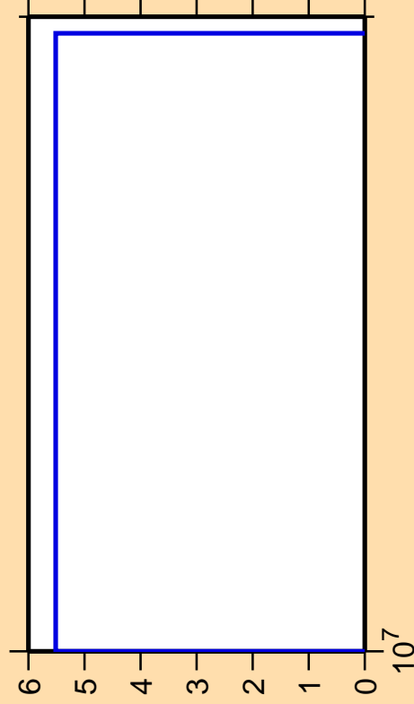
\Delta\sigma/\sigma vs. E for ^{203}\text{Rn}(n,nt)
