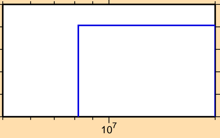
\sigma vs. E for ^{203}\text{Rn}(n,2np)
