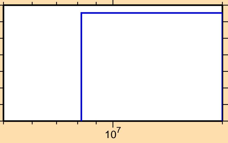
\sigma vs. E for ^{203}\text{Rn}(n,3n)
