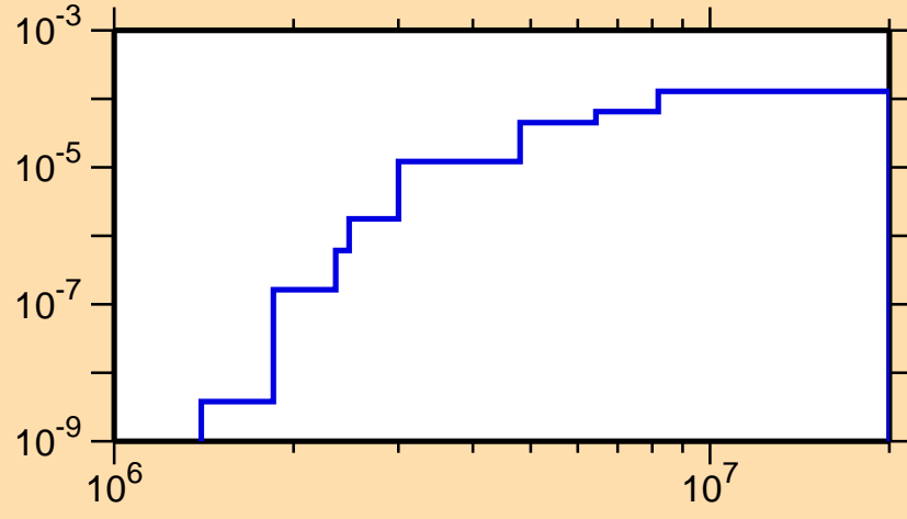
\sigma vs. E for ^{203}\text{Rn}(n,n_3)
