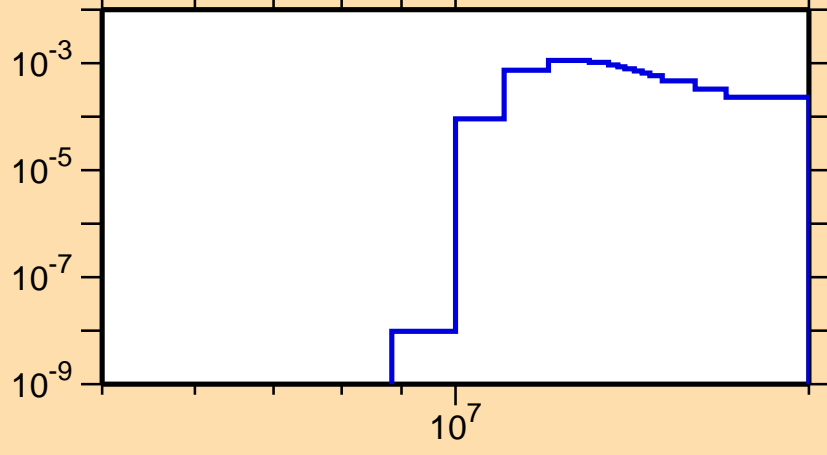
\sigma vs. E for ^{203}\text{Rn}(n,2n\alpha)
