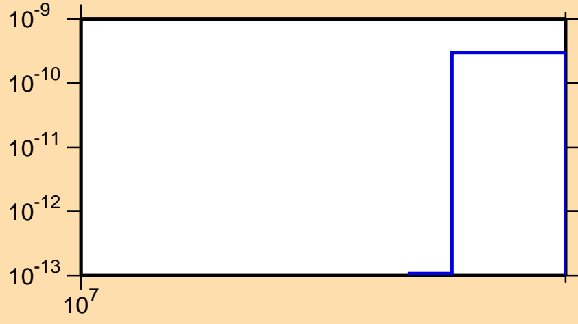
\sigma vs. E for ^{203}\text{Rn}(n,nt)
