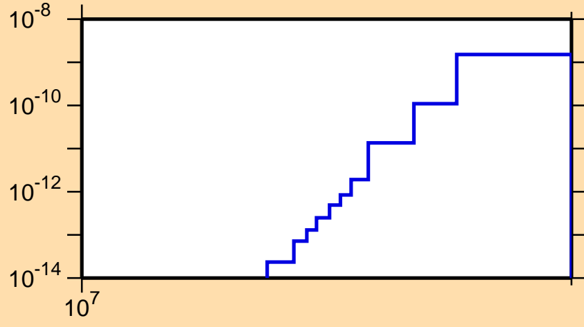
\sigma vs. E for ^{203}\text{Rn} (mt 34)
