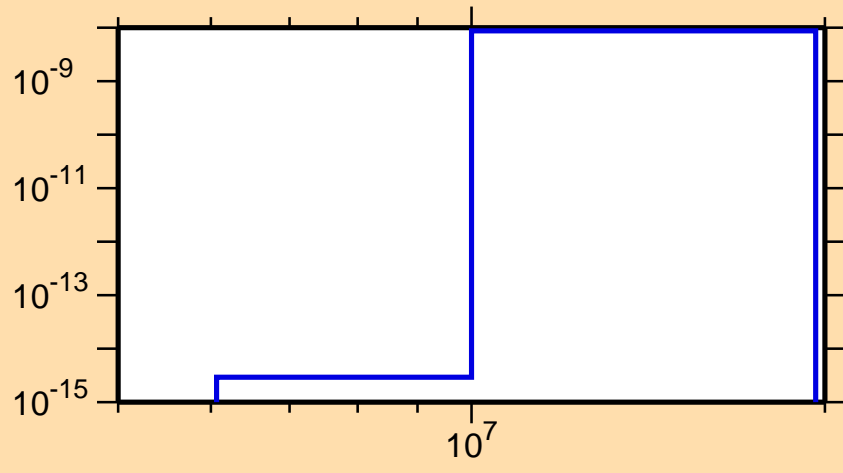
\sigma vs. E for ^{203}\text{Rn} (mt 45)
