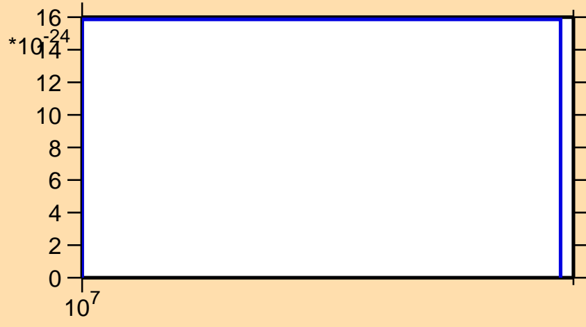
\sigma vs. E for ^{203}\text{Rn} (mt 11)
