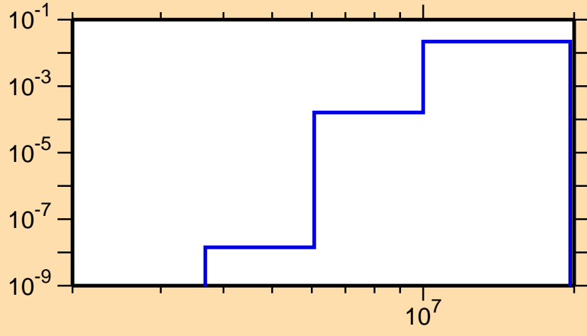
\sigma vs. E for ^{203}\text{Rn}(n,np)
