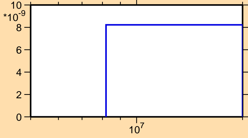
\sigma vs. E for ^{203}\text{Rn}(n,\text{pd})
