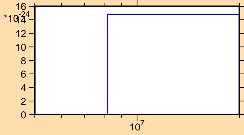
\sigma vs. E for ^{203}\text{Rn}(\text{mt 11})
