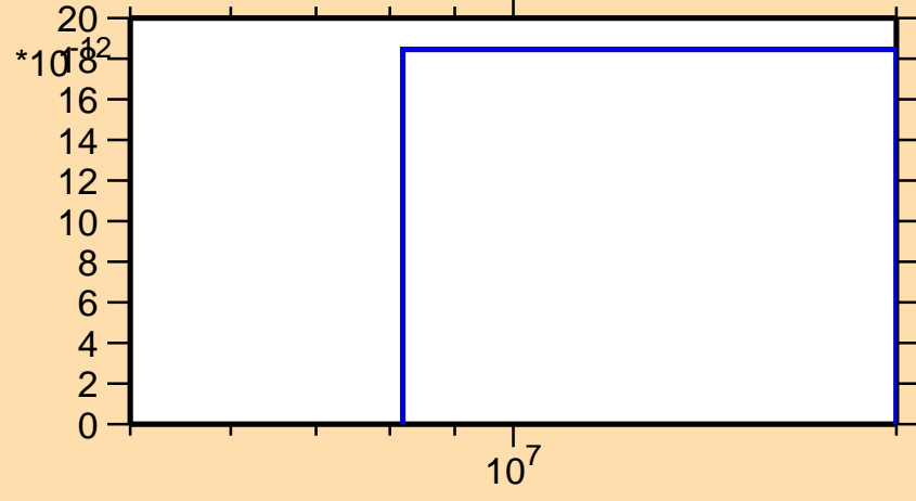
\sigma vs. E for ^{203}\text{Rn}(\text{mt } 34)
