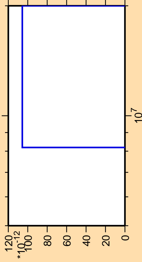
\Delta\sigma/\sigma vs. E for ^{203}\text{Rn}(\text{mt 11})
