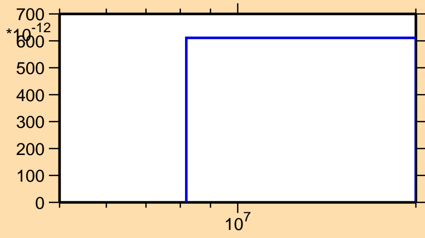
\sigma vs. E for ^{203}\text{Rn}(n,pt)
