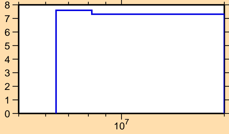
\Delta\sigma/\sigma vs. E for ^{203}\text{Rn}(n,\text{nonel.})
