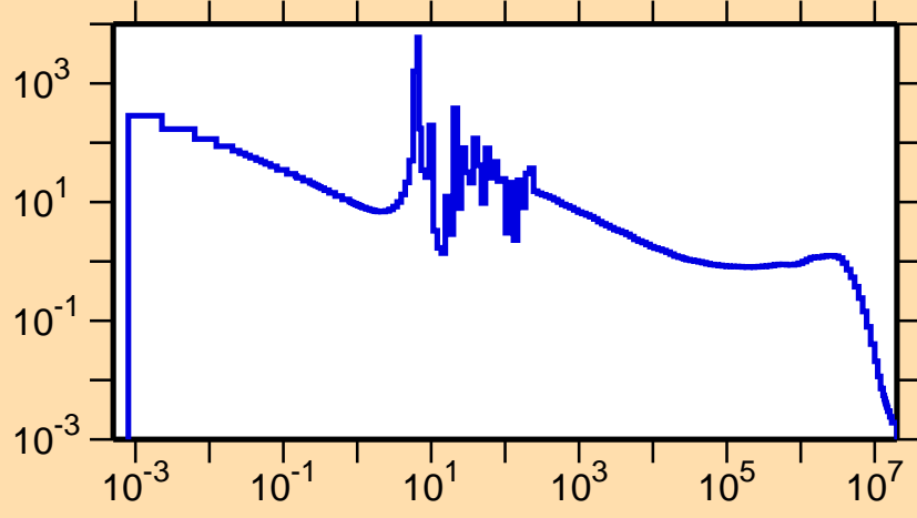
\sigma vs. E for ^{204}\text{Rn}(n,\gamma)
