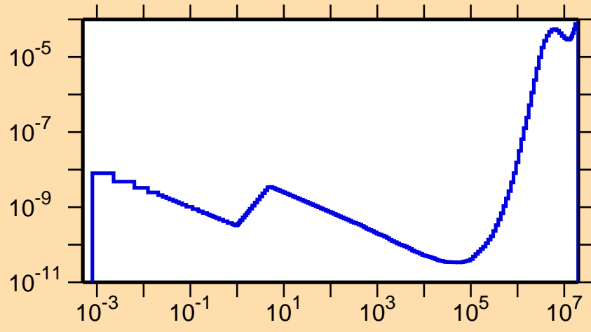
\sigma vs. E for ^{204}\text{Rn}(n,p\alpha)
