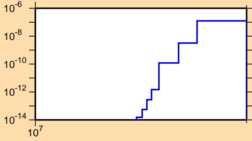
\sigma vs. E for ^{204}\text{Rn}(n,\text{nd})
