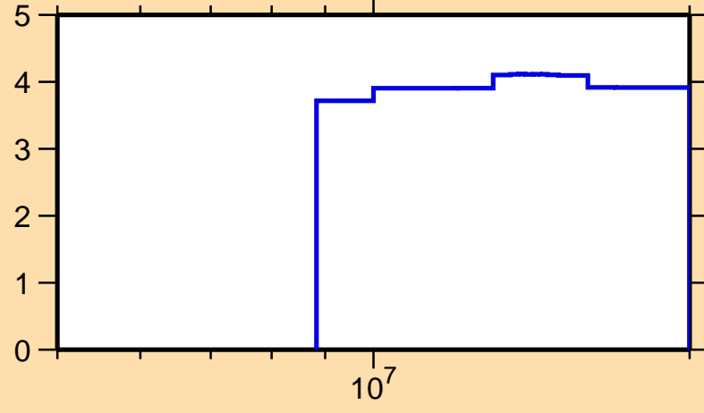
\Delta\sigma/\sigma vs. E for ^{204}\text{Rn}(n,\text{el.})
