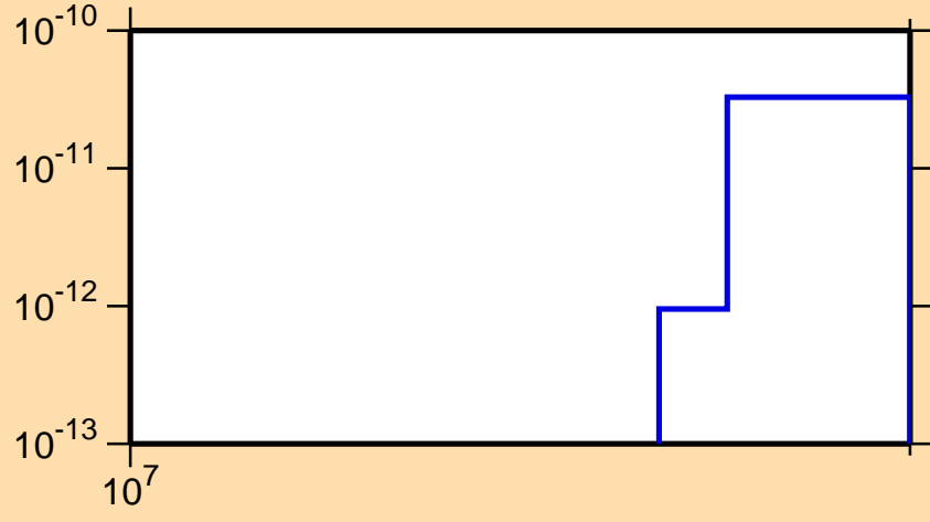
\sigma vs. E for ^{204}\text{Rn} (mt 34)
