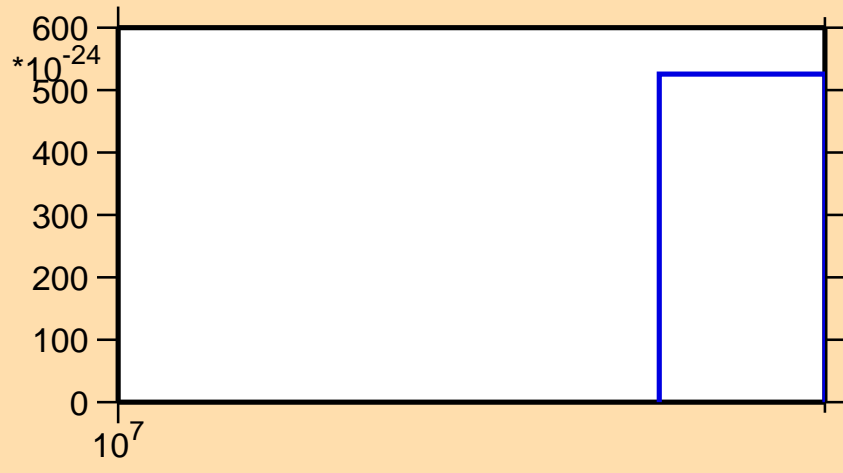
\sigma vs. E for ^{204}\text{Rn}(\text{mt 11})
