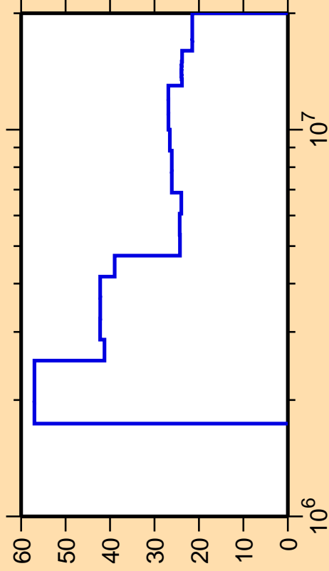
\Delta\sigma/\sigma vs. E for ^{204}\text{Rn}(n,n_4)
