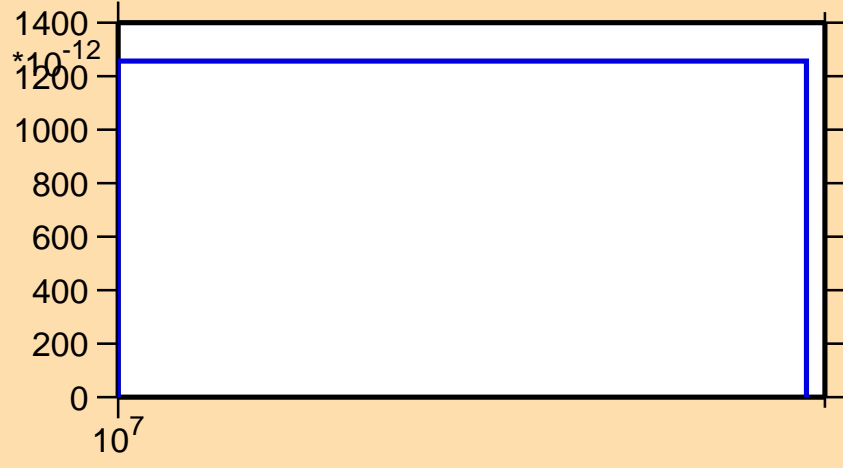
\sigma vs. E for ^{204}\text{Rn}(n,nd)
