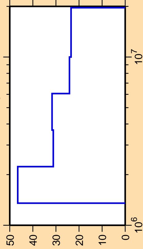
\Delta\sigma/\sigma vs. E for ^{204}\text{Rn}(n,n_3)
