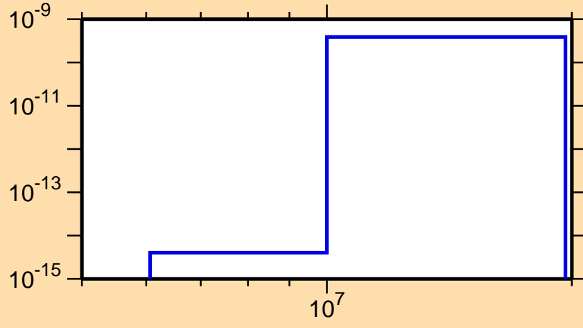
\sigma vs. E for ^{204}\text{Rn}(\text{mt117})
