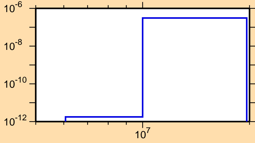
\sigma vs. E for ^{204}\text{Rn}(n,\text{He3})
