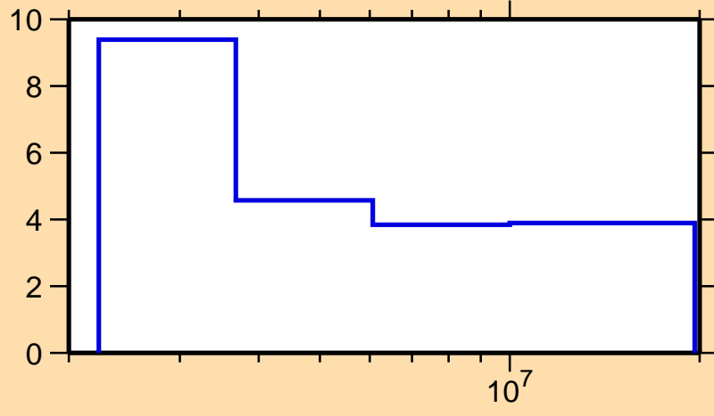
\Delta\sigma/\sigma vs. E for ^{204}\text{Rn}(n,\text{nonel.})
