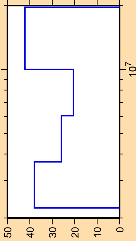
\Delta\sigma/\sigma vs. E for ^{204}\text{Rn}(n,n\text{cont.})
