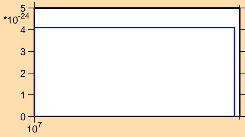
\sigma vs. E for ^{204}\text{Rn} (mt 11)
