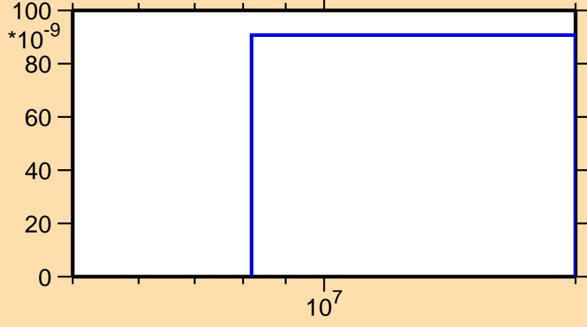
\sigma vs. E for ^{204}\text{Rn}(n,3n)
