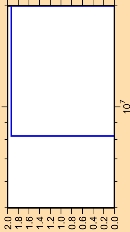
\Delta\sigma/\sigma vs. E for ^{204}\text{Rn}(\text{mt } 34)
