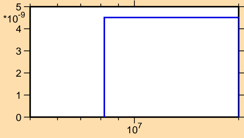
\sigma vs. E for ^{204}\text{Rn}(n,\text{pd})
