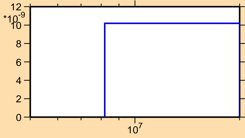
\sigma vs. E for ^{204}\text{Rn}(\text{mt } 45)
