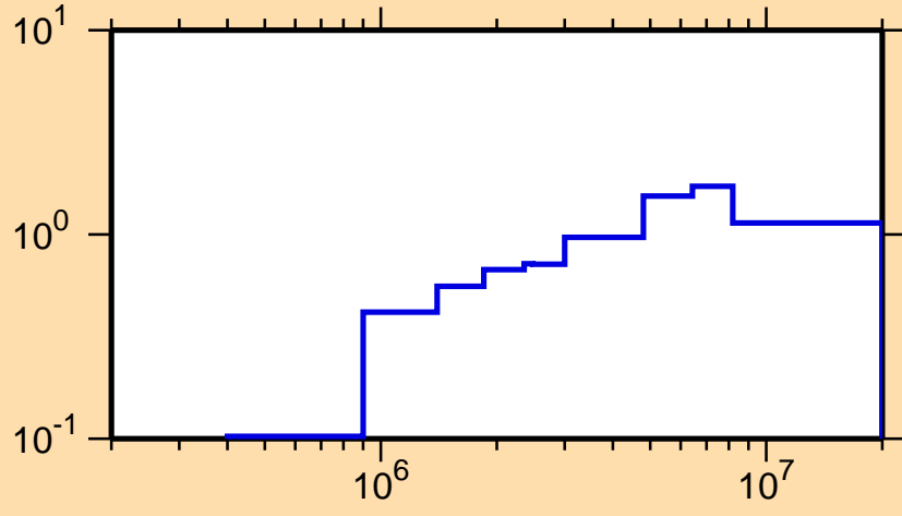
\sigma vs. E for ^{204}\text{Rn}(n,\text{inel.})
