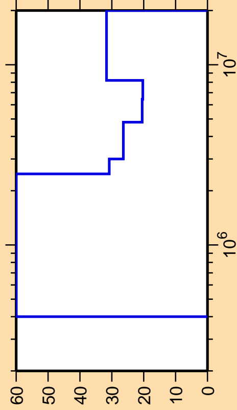
\Delta\sigma/\sigma vs. E for ^{204}\text{Rn}(n,\text{inel.})
