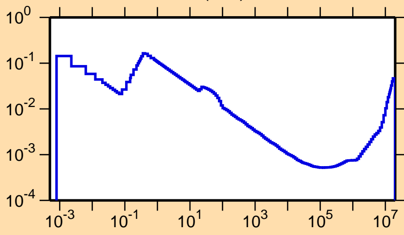
\sigma vs. E for ^{205}\text{Rn}(n,\alpha)
