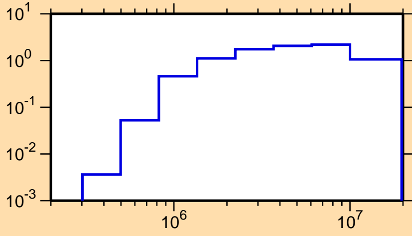
\sigma vs. E for ^{205}\text{Rn}(n,\text{inel.})
