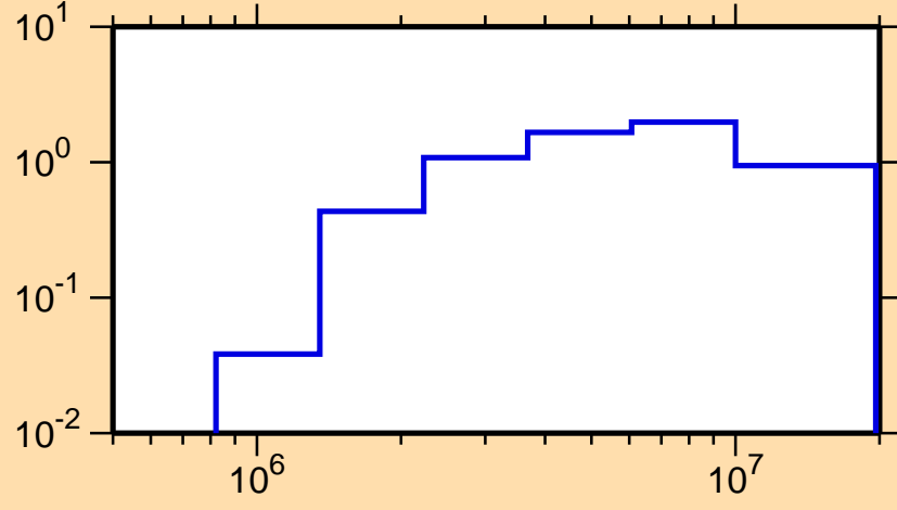
\sigma vs. E for ^{205}\text{Rn}(n,n\text{cont.})
