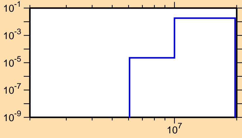
\sigma vs. E for ^{205}\text{Rn}(n,np)
