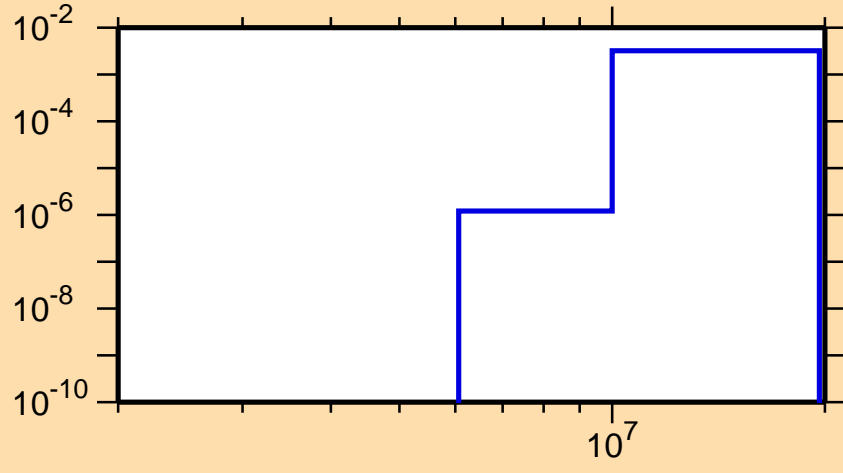
\sigma vs. E for ^{205}\text{Rn}(n,d)
