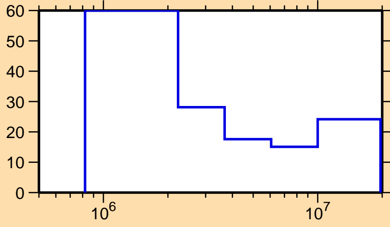
\Delta\sigma/\sigma vs. E for ^{205}\text{Rn}(n,n\text{cont.})
