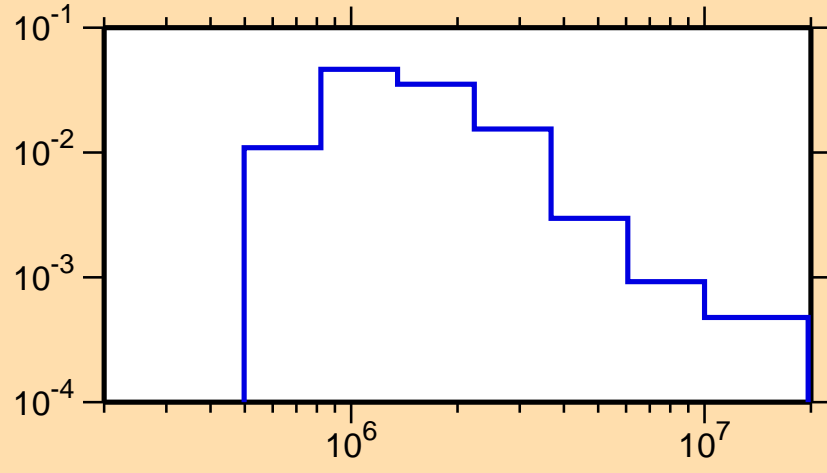
\sigma vs. E for ^{205}\text{Rn}(n,n_2)
