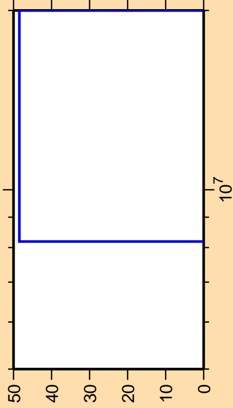
\Delta\sigma/\sigma vs. E for ^{205}\text{Rn}(\text{mt } 34)
