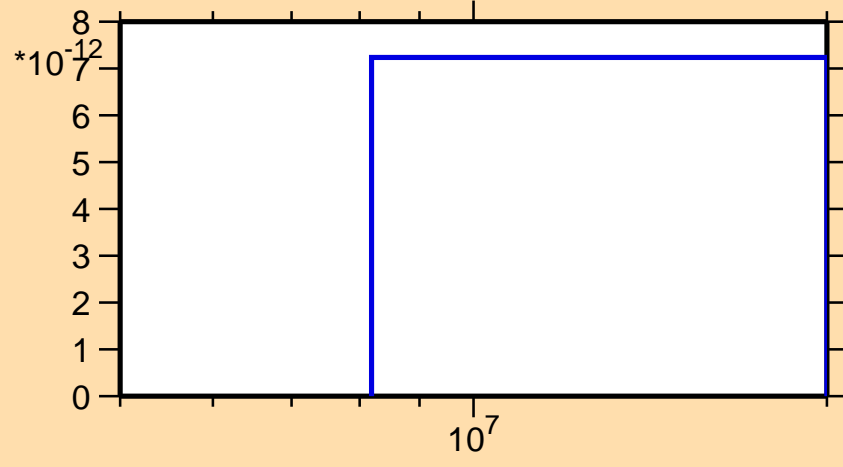
\sigma vs. E for ^{205}\text{Rn}(\text{mt } 34)
