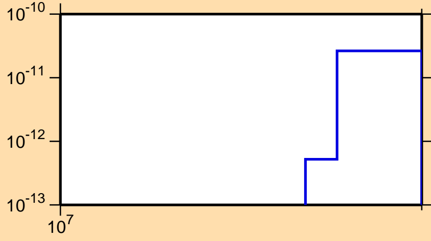
\sigma vs. E for ^{206}\text{Rn} (mt 34)
