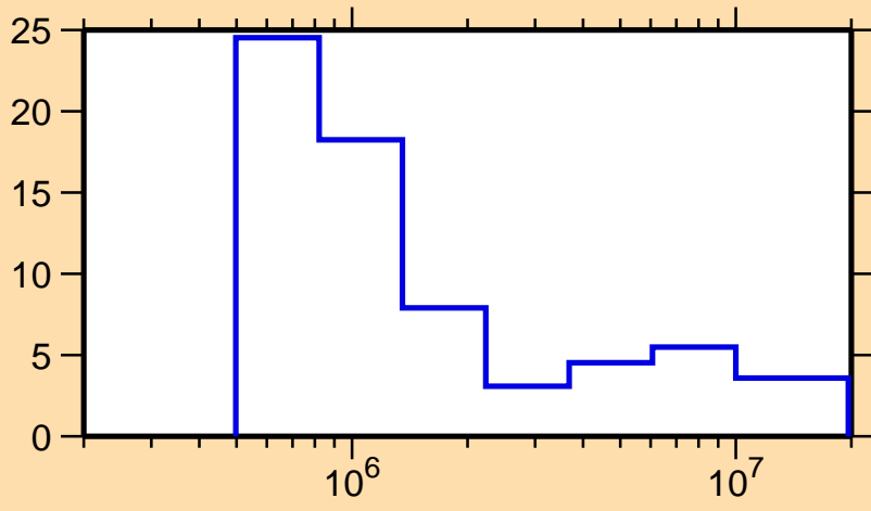
\Delta\sigma/\sigma vs. E for ^{206}\text{Rn}(n,\text{tot.})
