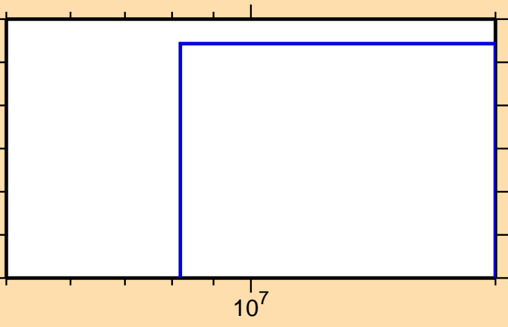
\sigma vs. E for ^{206}\text{Rn}(n,2np)
