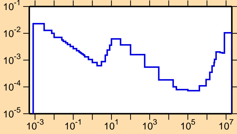
\sigma vs. E for ^{206}\text{Rn}(n,\alpha)
