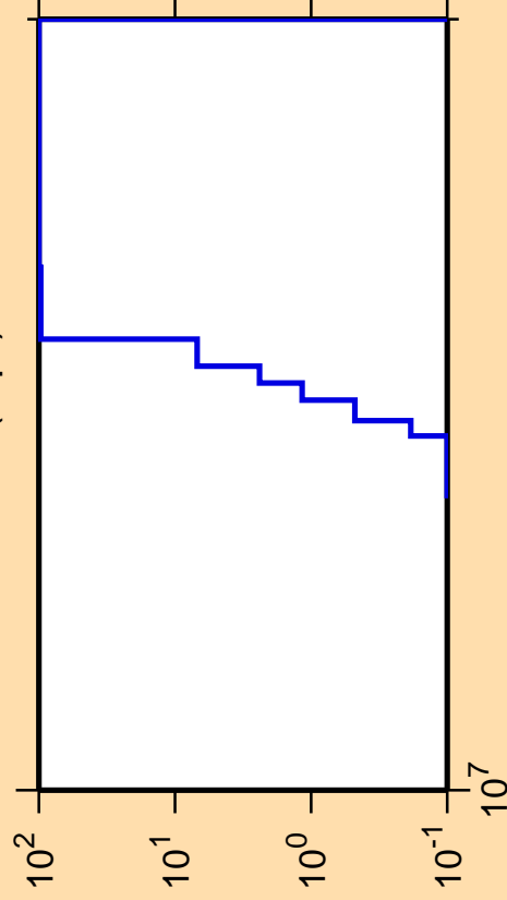
\Delta\sigma/\sigma vs. E for ^{207}\text{Rn}(n,pt)
