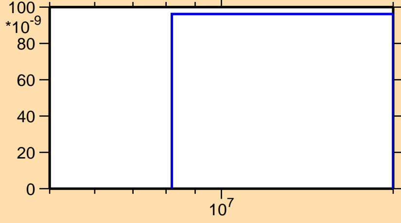
\sigma vs. E for ^{207}\text{Rn}(n,nd)
