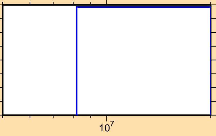
\sigma vs. E for ^{207}\text{Rn}(\text{mt117})
