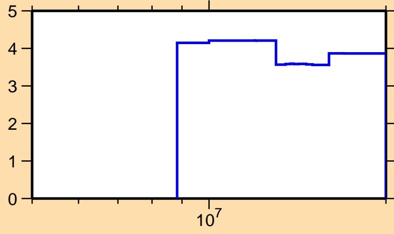
\Delta\sigma/\sigma vs. E for ^{208}\text{Rn}(n,\text{nonel.})
