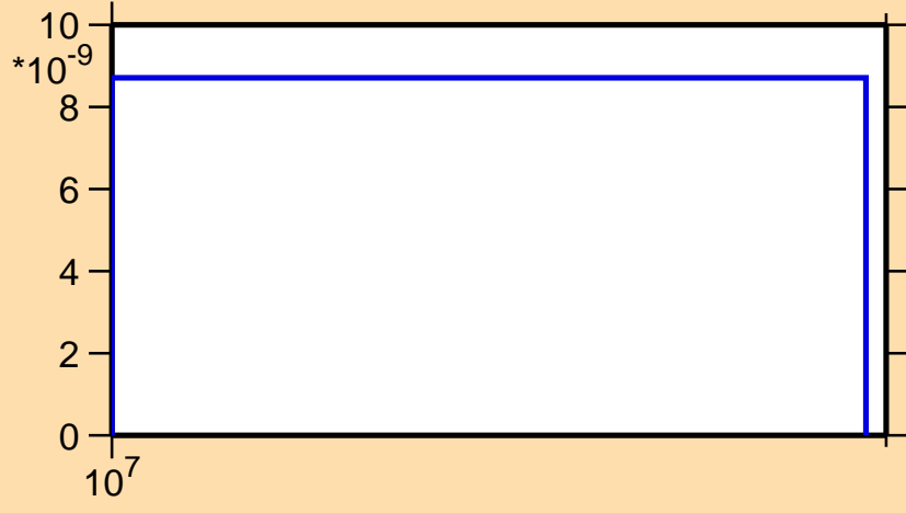
\sigma vs. E for ^{208}\text{Rn}(n,\text{nd})
