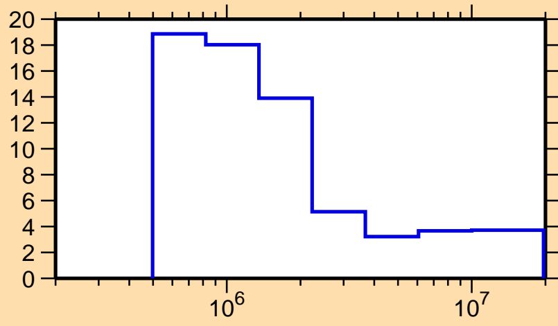
\Delta\sigma/\sigma vs. E for ^{208}\text{Rn}(n,\text{nonel.})
