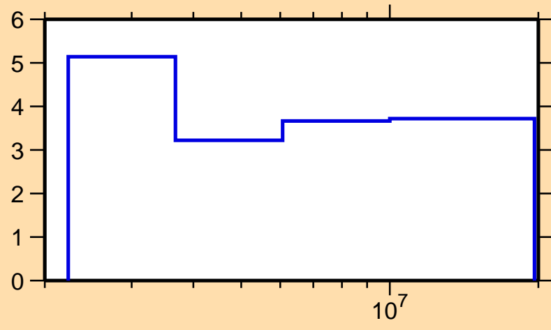
\Delta\sigma/\sigma vs. E for ^{208}\text{Rn}(n,n\text{onel.})
