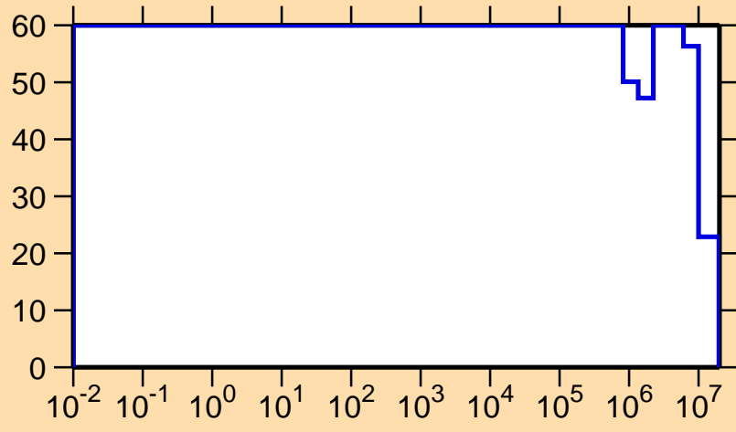
\Delta\sigma/\sigma vs. E for ^{208}\text{Rn}(n,p)
