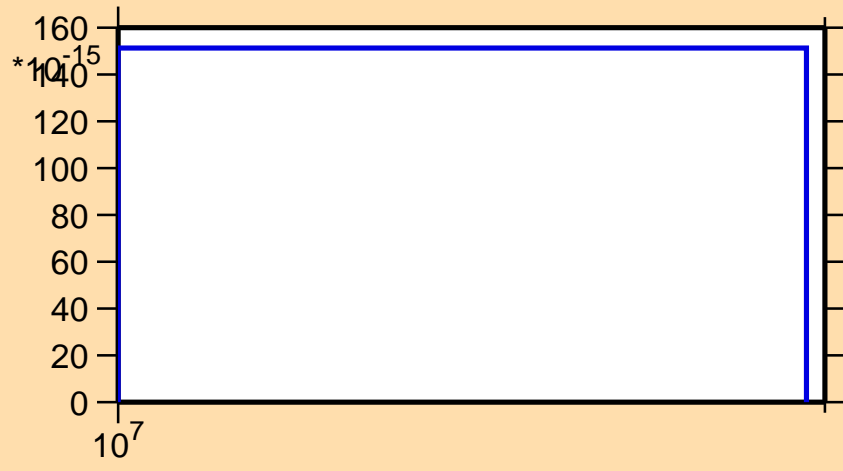
\sigma vs. E for ^{208}\text{Rn} (mt 34)
