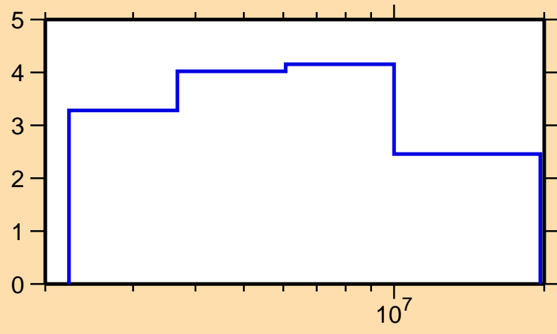
\Delta\sigma/\sigma vs. E for ^{208}\text{Rn}(n,\text{el.})
