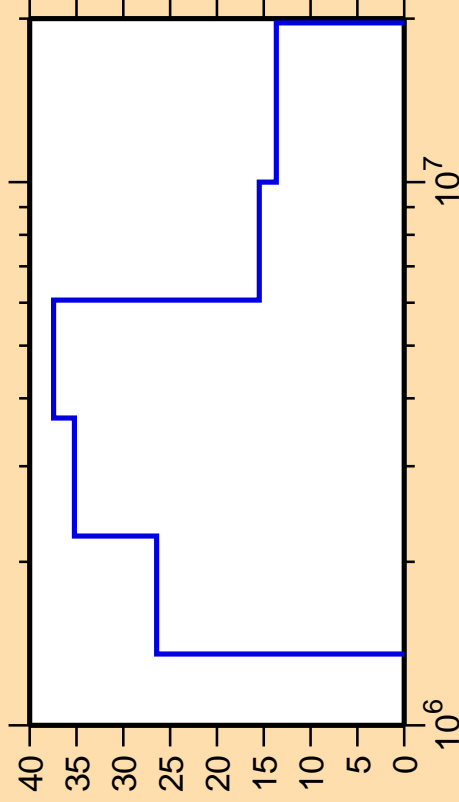
\Delta\sigma/\sigma vs. E for ^{208}\text{Rn}(n,n_3)
