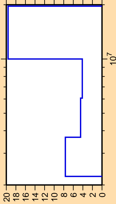
\Delta\sigma/\sigma vs. E for ^{208}\text{Rn}(n,n\text{cont.})
