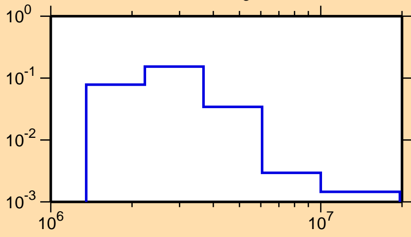
\sigma vs. E for ^{208}\text{Rn}(n,n_3)
