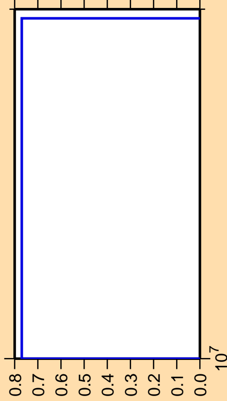
\Delta\sigma/\sigma vs. E for ^{208}\text{Rn} (mt 34)
