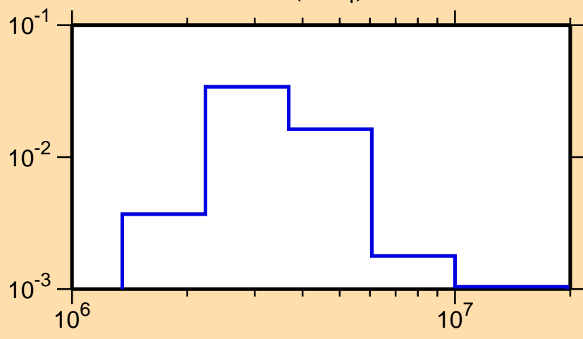
\sigma vs. E for ^{208}\text{Rn}(n,n_4)
