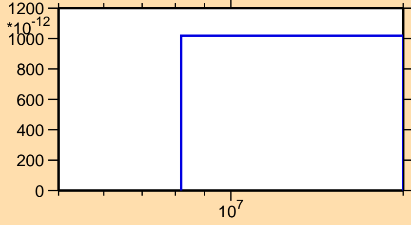
\sigma vs. E for ^{208}\text{Rn}(\text{mt } 45)
