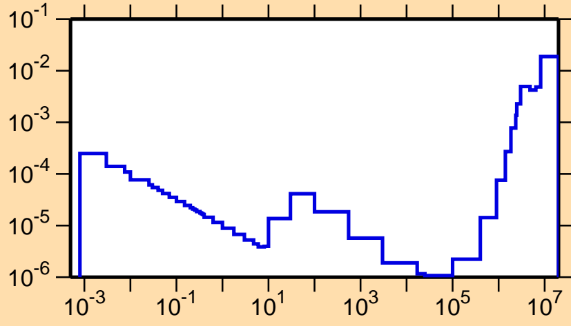
\sigma vs. E for ^{208}\text{Rn}(n,p)
