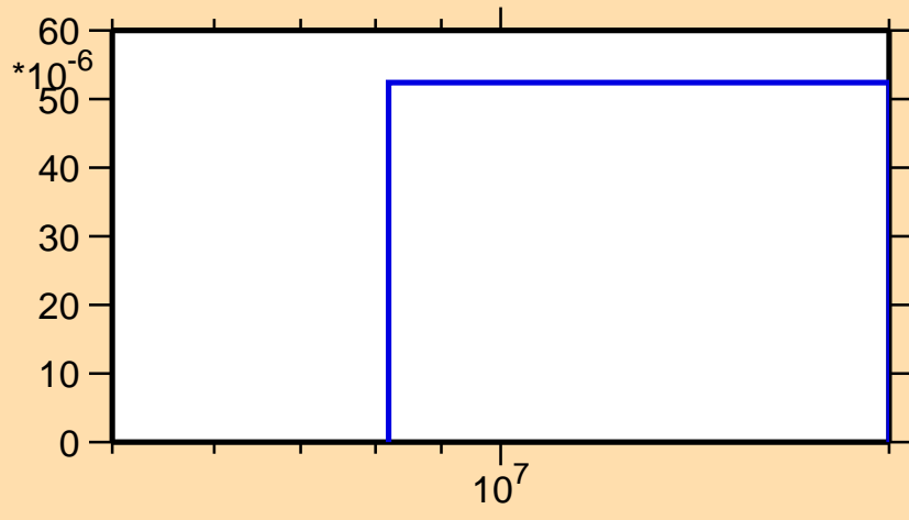
\sigma vs. E for ^{208}\text{Rn}(n,t)
