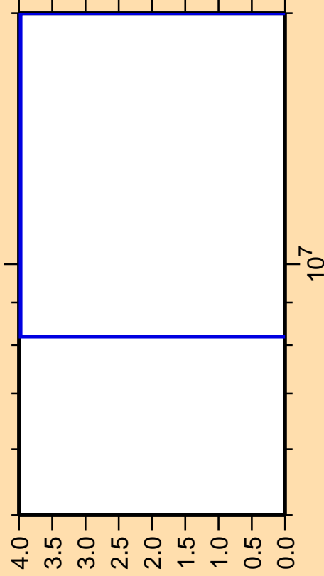
\Delta\sigma/\sigma vs. E for ^{208}\text{Rn}(n,pt)
