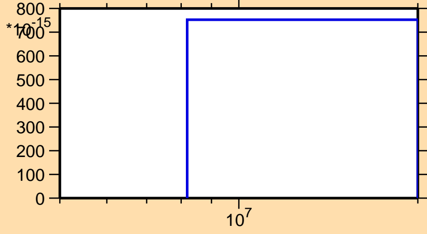
\sigma vs. E for ^{208}\text{Rn}(n,pt)
