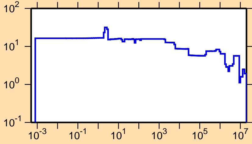
\Delta\sigma/\sigma vs. E for ^{209}\text{Rn}(n,\text{el.})
