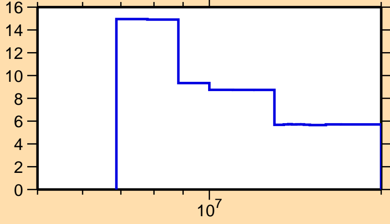
\Delta\sigma/\sigma vs. E for ^{209}\text{Rn}(n,2n)
