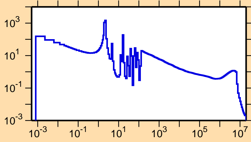
\sigma vs. E for ^{209}\text{Rn}(n,\gamma)
