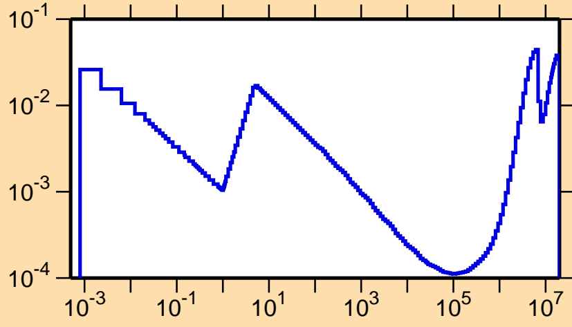
\sigma vs. E for ^{209}\text{Rn}(n,p)
