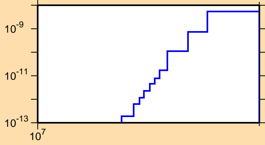
\sigma vs. E for ^{209}\text{Rn}(n,\text{pd})
