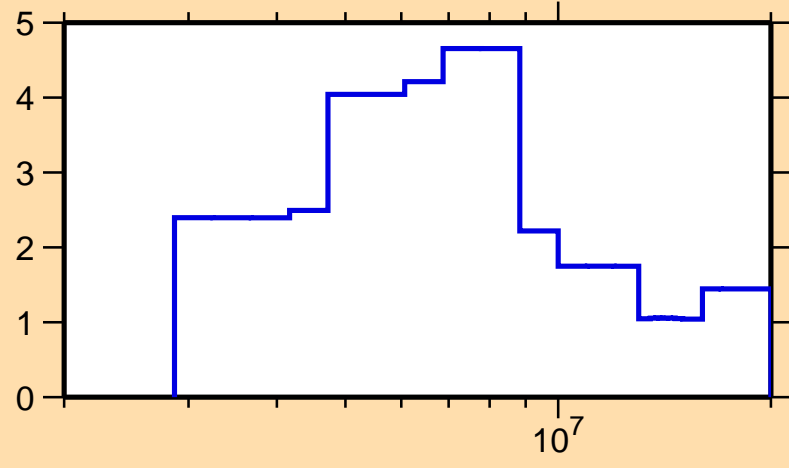
\Delta\sigma/\sigma vs. E for ^{209}\text{Rn}(n,\text{tot.})
