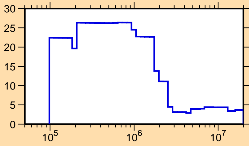
\Delta\sigma/\sigma vs. E for ^{209}\text{Rn}(n,\text{nonel.})
