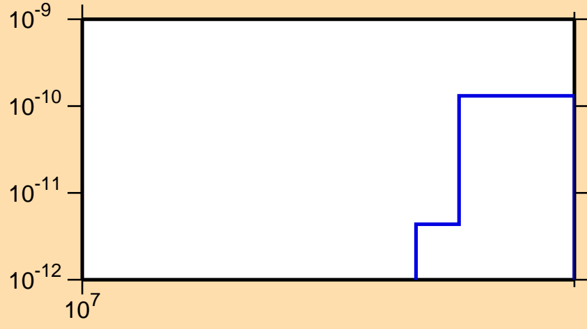
\sigma vs. E for ^{209}\text{Rn} (mt 34)
