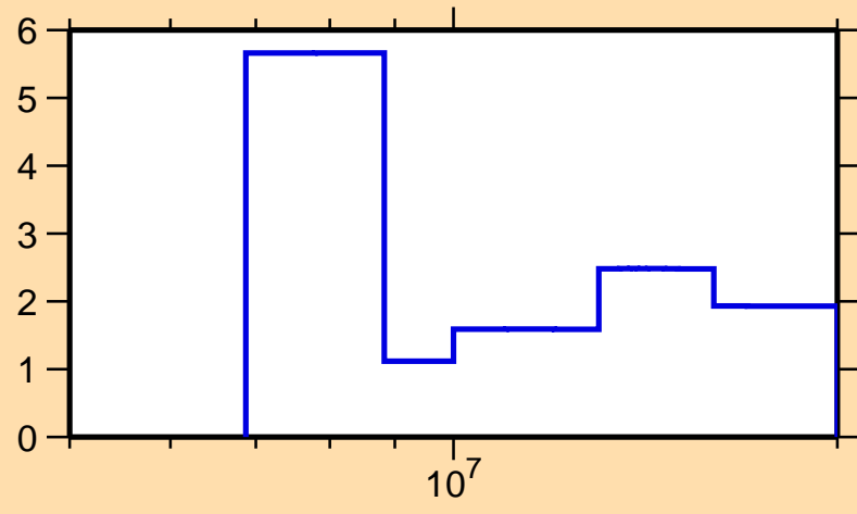
\Delta\sigma/\sigma vs. E for ^{209}\text{Rn}(n,\text{el.})
