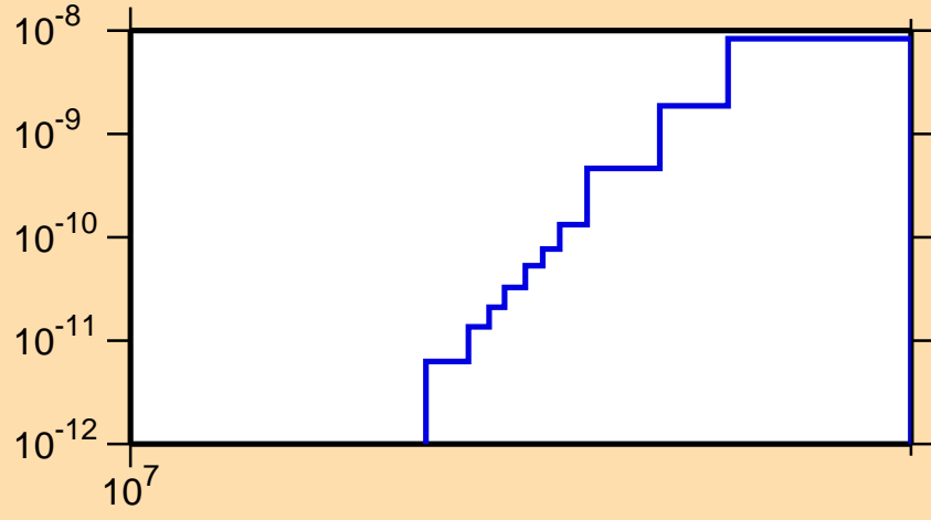
\sigma vs. E for ^{209}\text{Rn} (mt 45)
