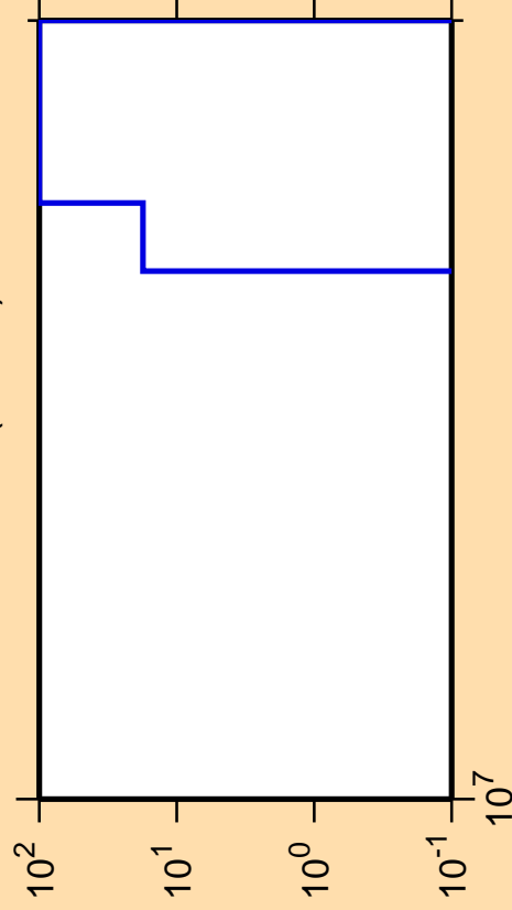
\Delta\sigma/\sigma vs. E for ^{209}\text{Rn} (mt 34)
