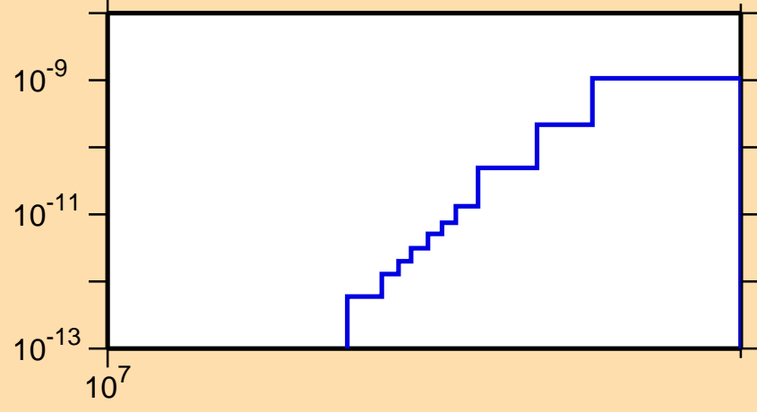
\sigma vs. E for ^{209}\text{Rn}(\text{mt117})
