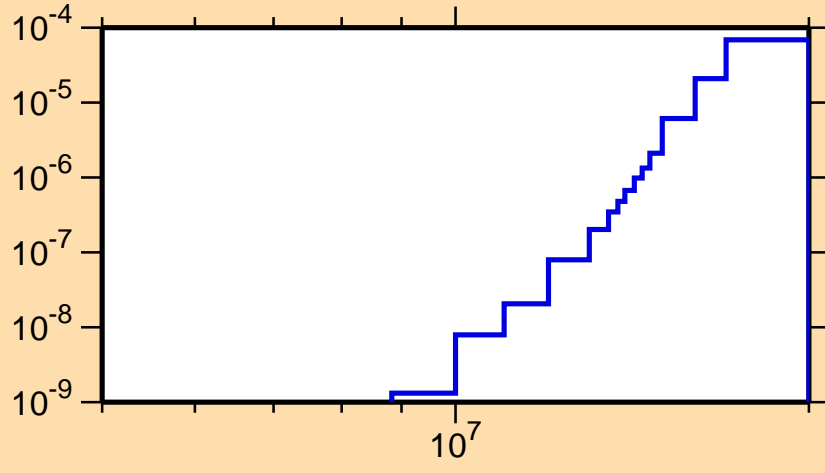
\sigma vs. E for ^{209}\text{Rn}(n,2n\alpha)
