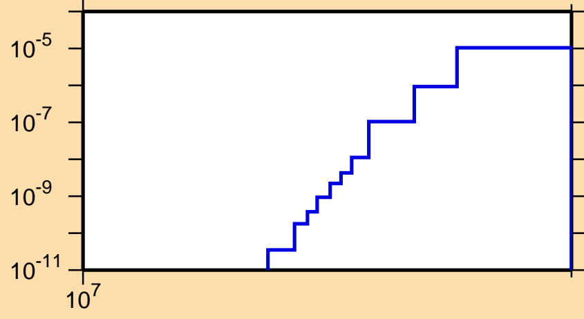
\sigma vs. E for ^{209}\text{Rn}(n,\text{nd})
