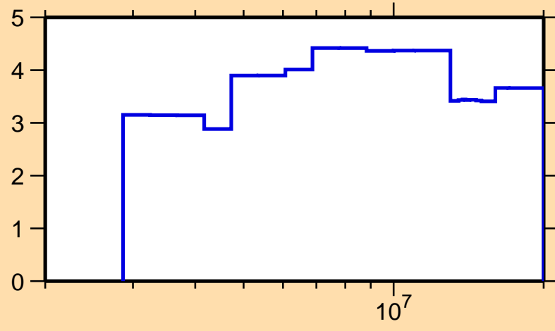
\Delta\sigma/\sigma vs. E for ^{209}\text{Rn}(n,n\text{onel.})
