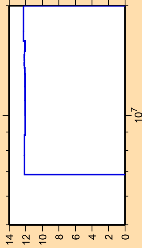
\Delta\sigma/\sigma vs. E for ^{209}\text{Rn}(n,n_1)
