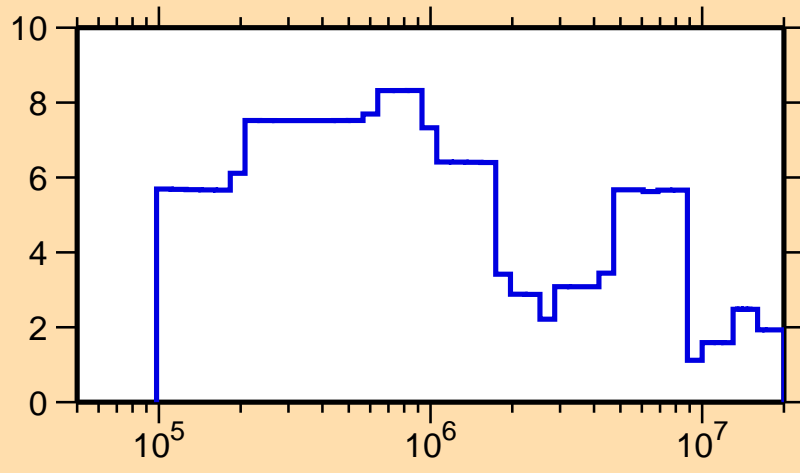
\Delta\sigma/\sigma vs. E for ^{209}\text{Rn}(n,\text{el.})
