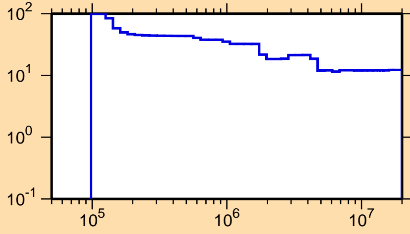
\Delta\sigma/\sigma vs. E for ^{209}\text{Rn}(n,n_1)
