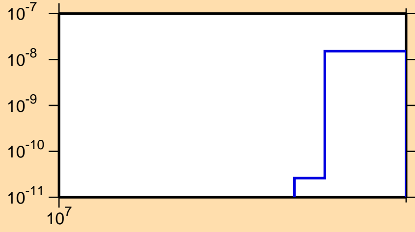
\sigma vs. E for ^{209}\text{Rn}(n,nt)
