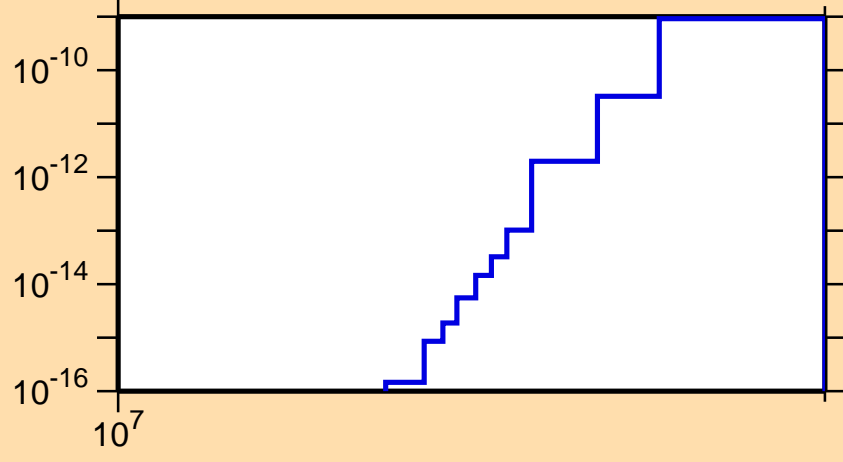
\sigma vs. E for ^{209}\text{Rn}(n,\text{pt})
