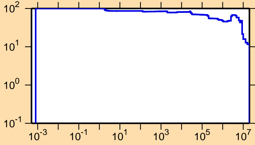
\Delta\sigma/\sigma vs. E for ^{209}\text{Rn}(n,p)
