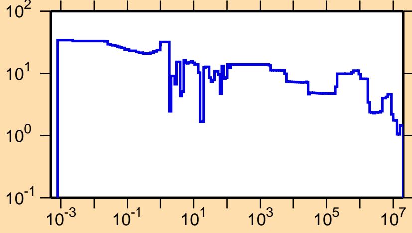
\Delta\sigma/\sigma vs. E for ^{209}\text{Rn}(n,\text{tot.})
