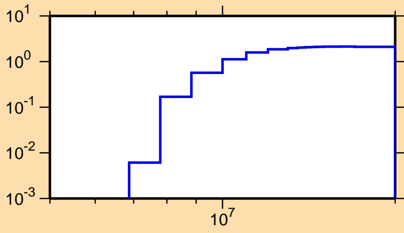
\sigma vs. E for ^{209}\text{Rn}(n,2n)
