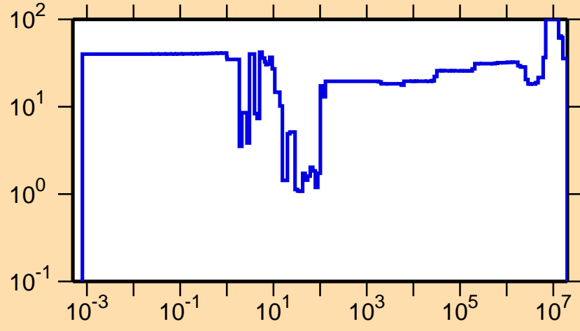
\Delta\sigma/\sigma vs. E for ^{209}\text{Rn}(n,\gamma)
