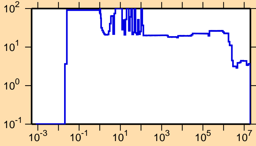
\Delta\sigma/\sigma vs. E for ^{209}\text{Rn}(n,\text{nonel.})
