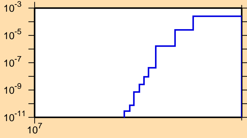
\sigma vs. E for ^{209}\text{Rn}(n,2np)
