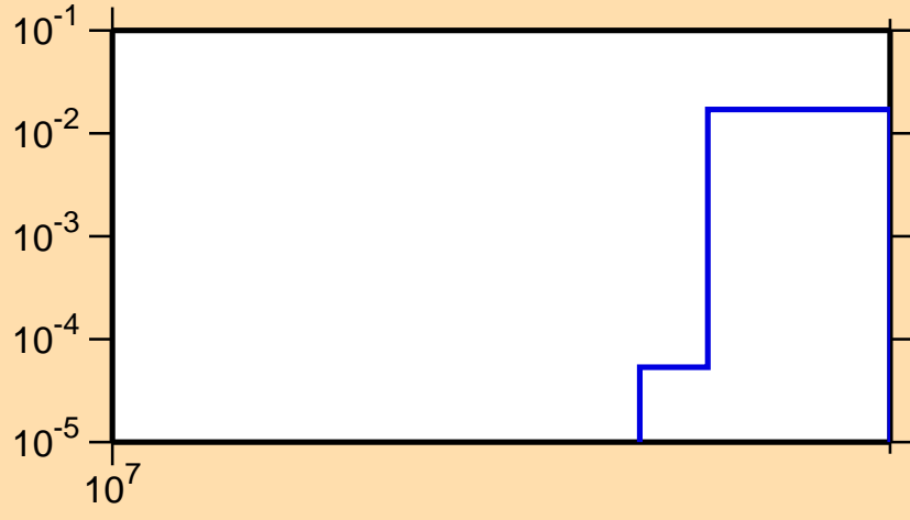
\sigma vs. E for ^{209}\text{Rn}(n,3n)
