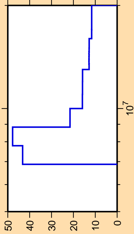
\Delta\sigma/\sigma vs. E for ^{209}\text{Rn}(n,p)
