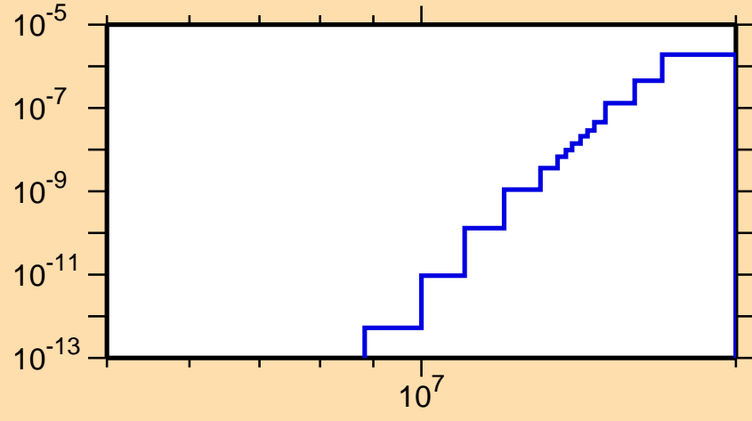
\sigma vs. E for ^{209}\text{Rn}(n,\text{He}3)
