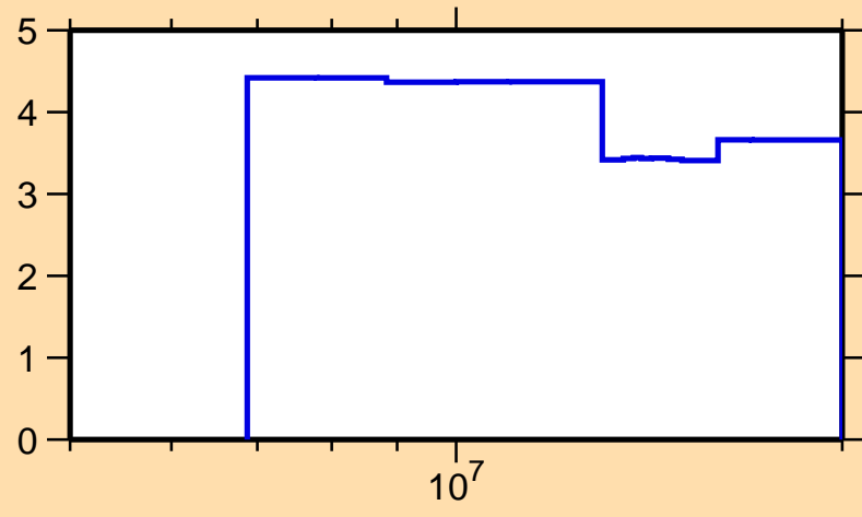
\Delta\sigma/\sigma vs. E for ^{209}\text{Rn}(n,\text{nonel.})
