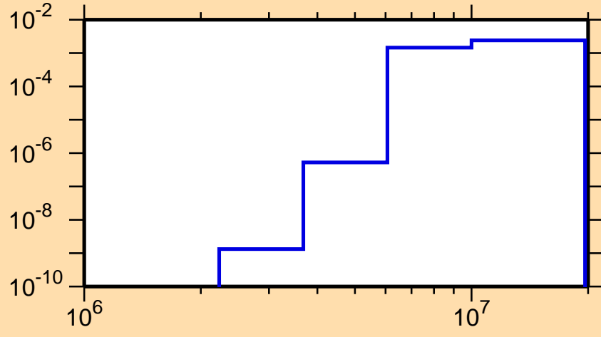
\sigma vs. E for ^{209}\text{Rn}(n,n\alpha)
