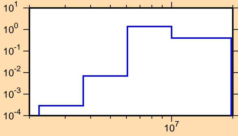
\sigma vs. E for ^{209}\text{Rn}(n,n\text{cont.})
