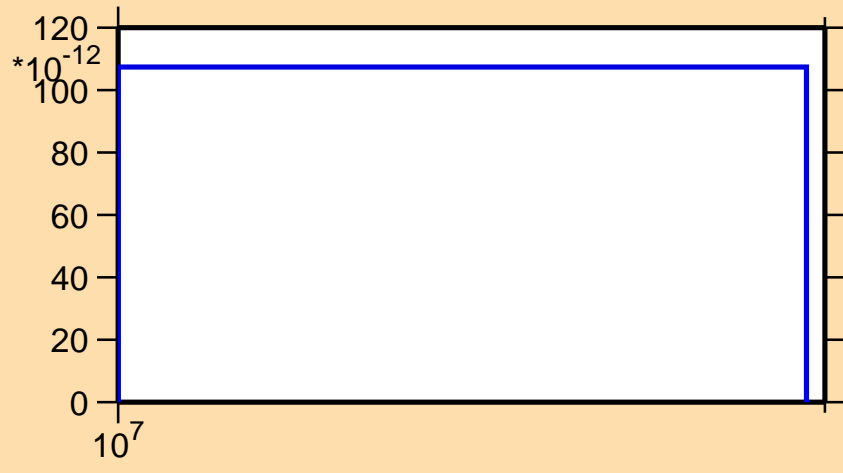
\sigma vs. E for ^{209}\text{Rn}(n,\text{pd})
