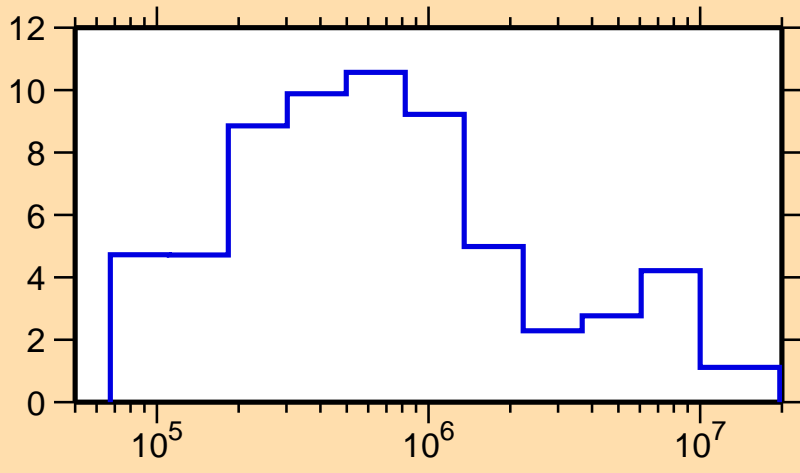
\Delta\sigma/\sigma vs. E for ^{209}\text{Rn}(n,\text{tot.})
