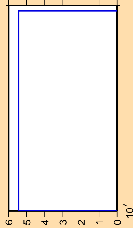
\Delta\sigma/\sigma vs. E for ^{209}\text{Rn} (mt 34)
