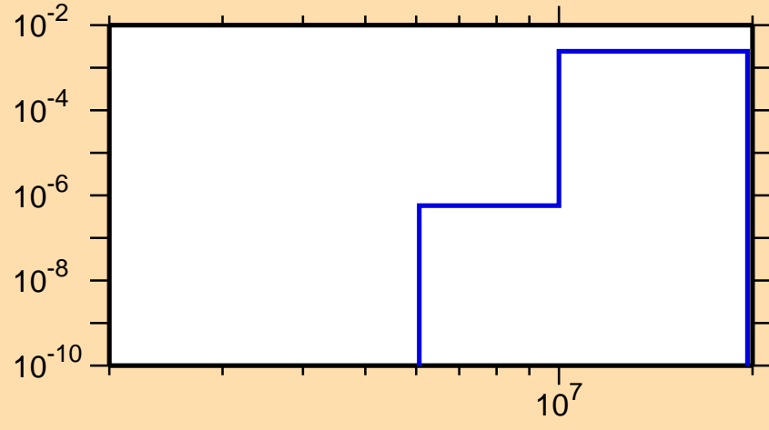
\sigma vs. E for ^{209}\text{Rn}(n,d)
