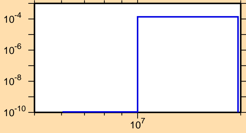
\sigma vs. E for ^{209}\text{Rn}(n,t)
