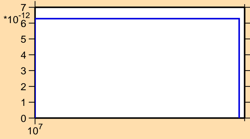
\sigma vs. E for ^{209}\text{Rn}(n,3n\alpha)
