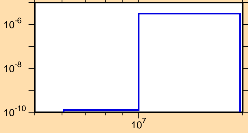
\sigma vs. E for ^{209}\text{Rn}(n,2n\alpha)
