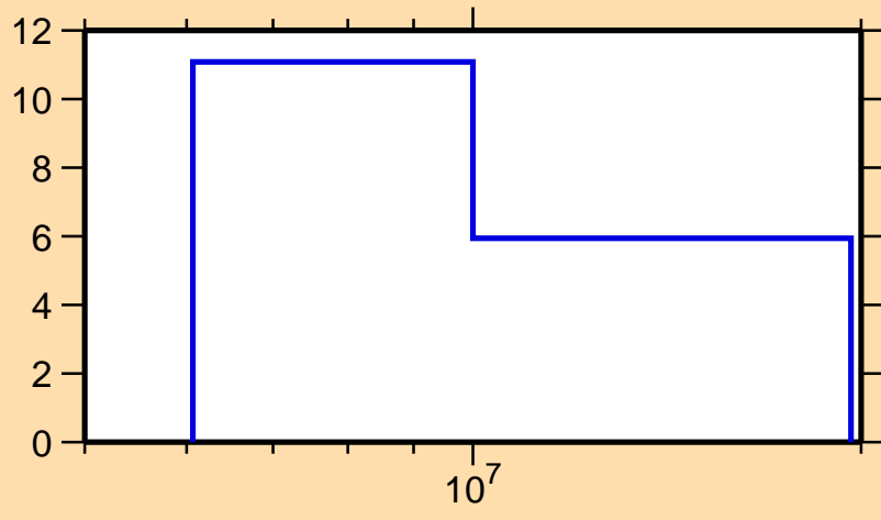
\Delta\sigma/\sigma vs. E for ^{209}\text{Rn}(n,2n)
