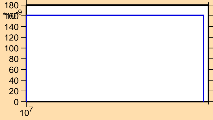
\sigma vs. E for ^{209}\text{Rn}(n,\text{nd})
