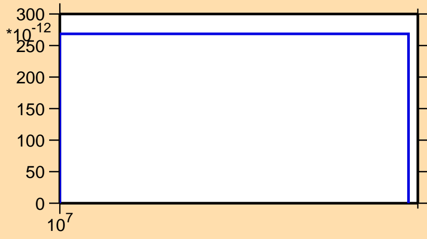
\sigma vs. E for ^{209}\text{Rn} (mt 45)
