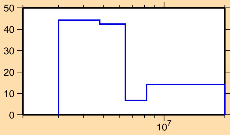
\Delta\sigma/\sigma vs. E for ^{209}\text{Rn}(n,n\text{cont.})
