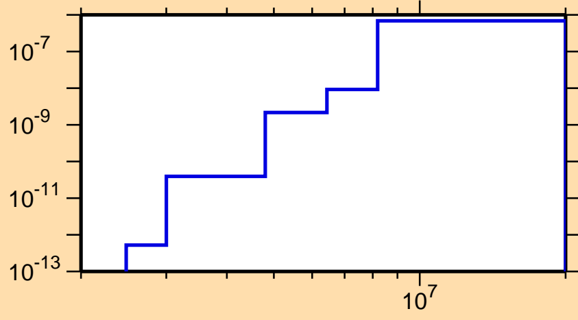
\sigma vs. E for ^{209}\text{Rn}(n,p\alpha)
