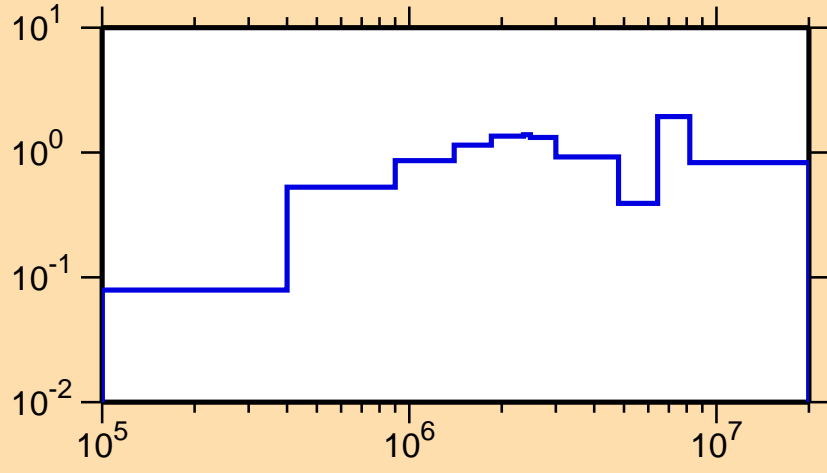
\sigma vs. E for ^{209}\text{Rn}(n,\text{inel.})
