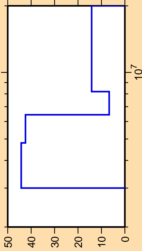
\Delta\sigma/\sigma vs. E for ^{209}\text{Rn}(n,n\text{cont.})
