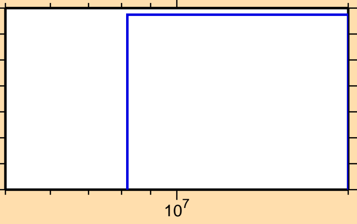
\sigma vs. E for ^{209}\text{Rn}(n,\text{nd})
