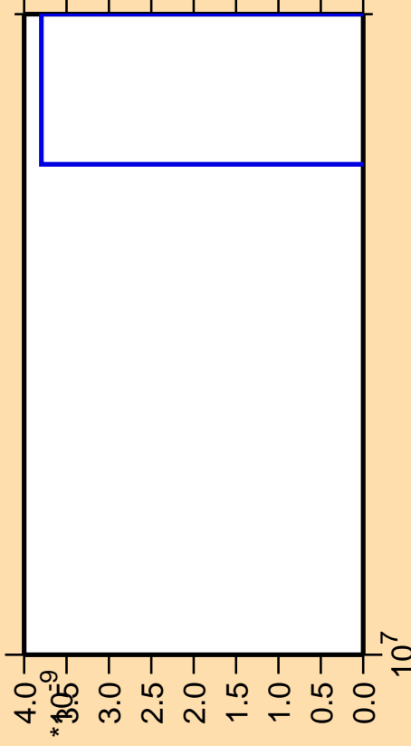
\Delta\sigma/\sigma vs. E for ^{210}\text{Rn} (mt 42)
