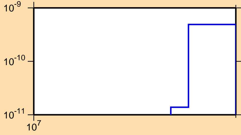
\sigma vs. E for ^{211}\text{Rn}(n,\text{pt})
