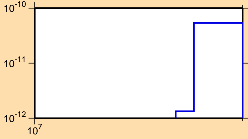
\sigma vs. E for ^{211}\text{Rn} (mt 34)
