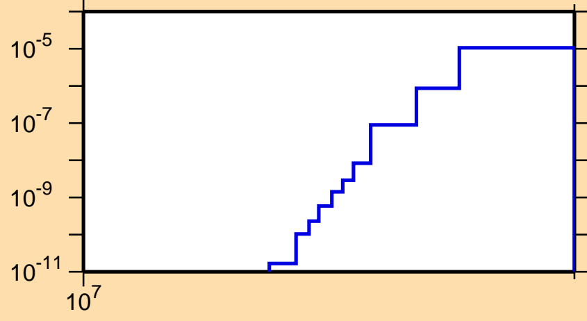
\sigma vs. E for ^{211}\text{Rn}(n,\text{nd})
